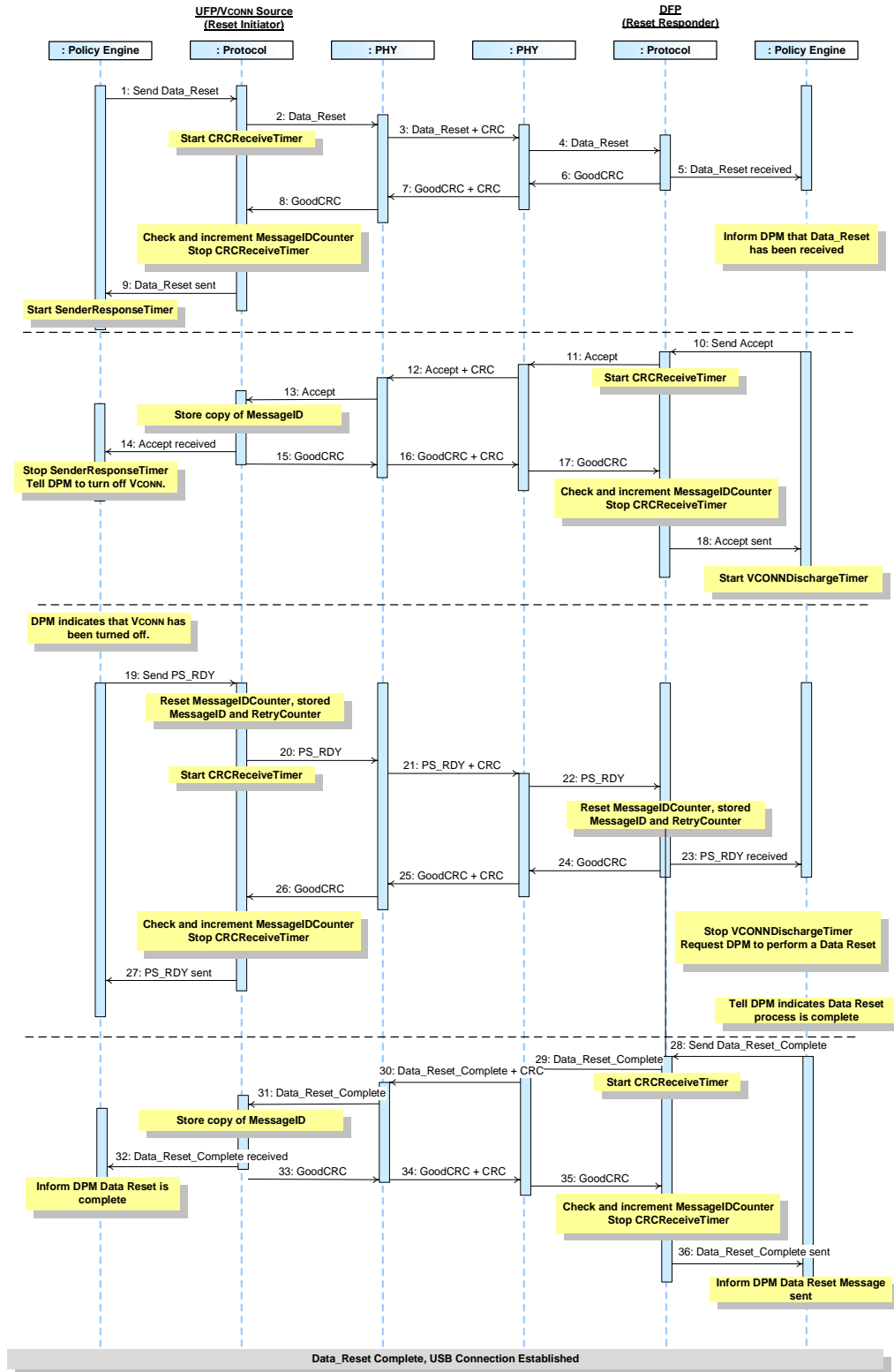
Figure 8-25 DFP Receives a Data Reset where the UFP is the VCONN Source
