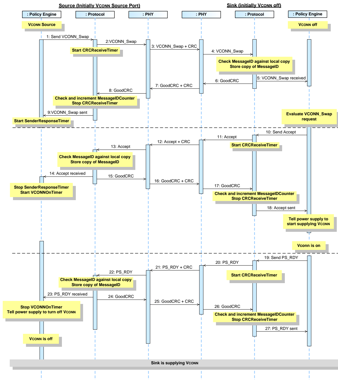
Figure 8-36 Source to Sink VCONN Source Swap
