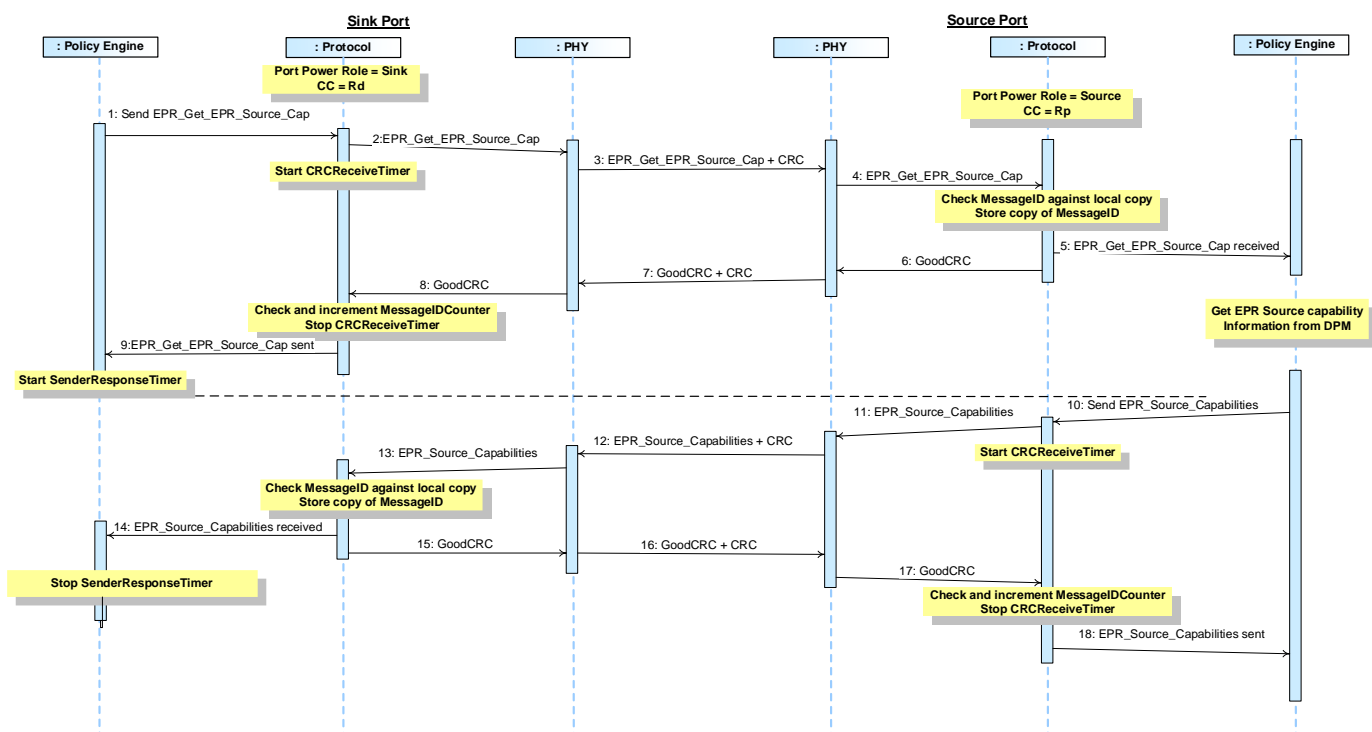
Figure 8-48 Sink Gets Source's EPR Capabilities
