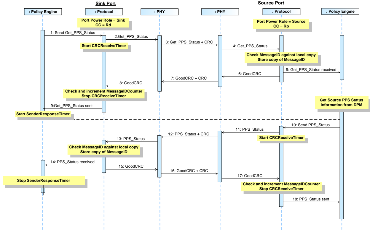
Figure 8-43 Sink Gets Source PPS Status
