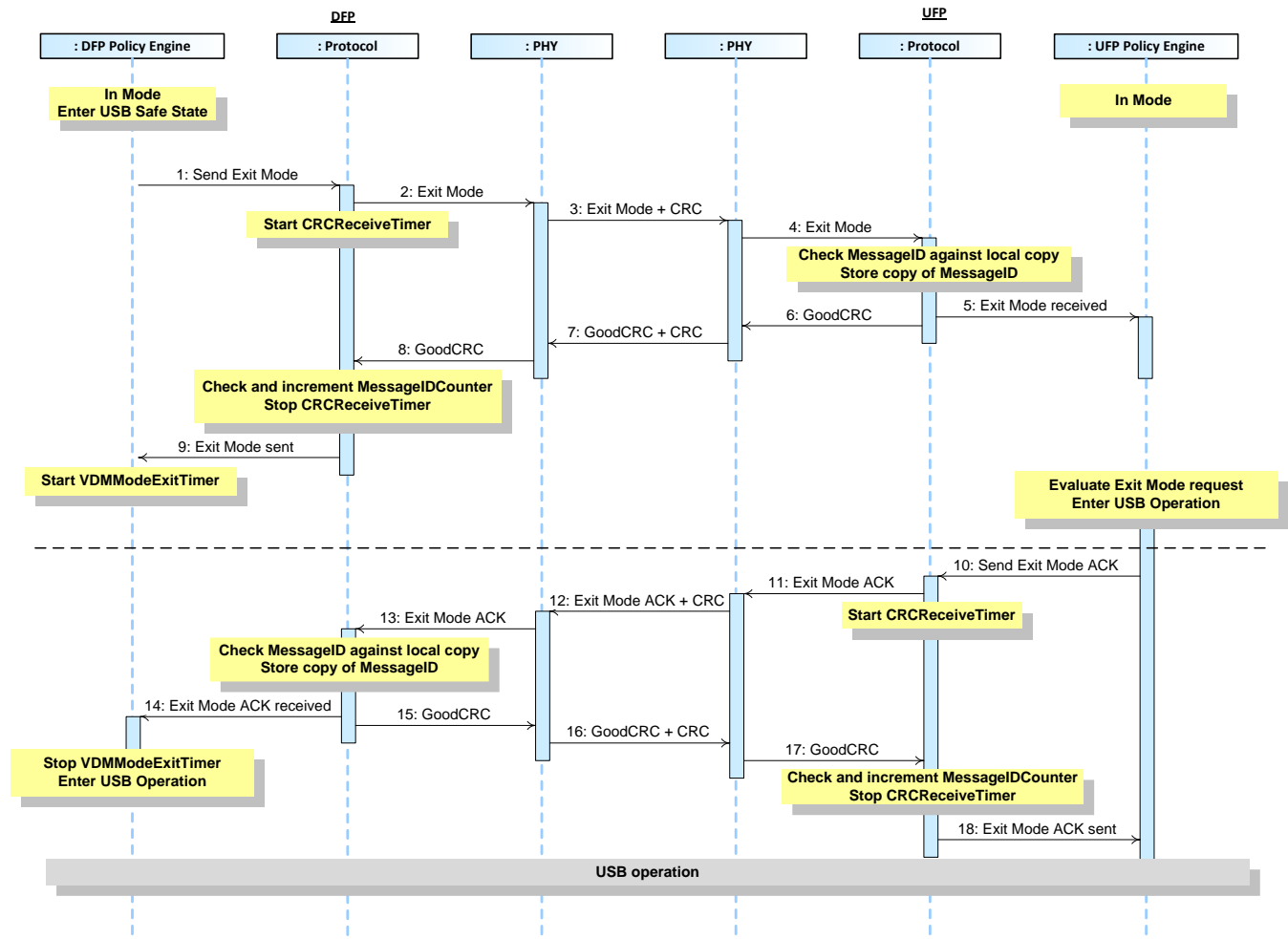
Figure 8-88 DFP to UFP Exit Mode
