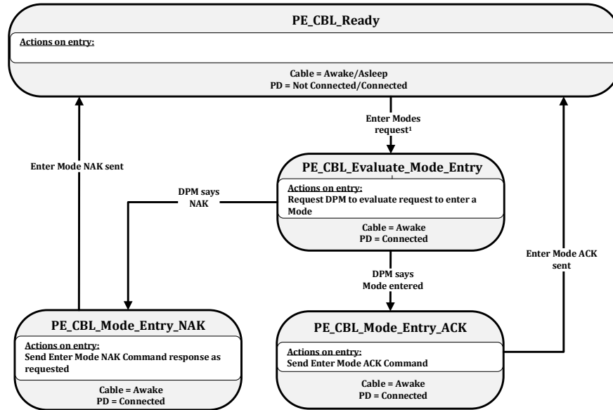
Figure 8-180 Cable Plug Structured VDM Enter Mode State Diagram
