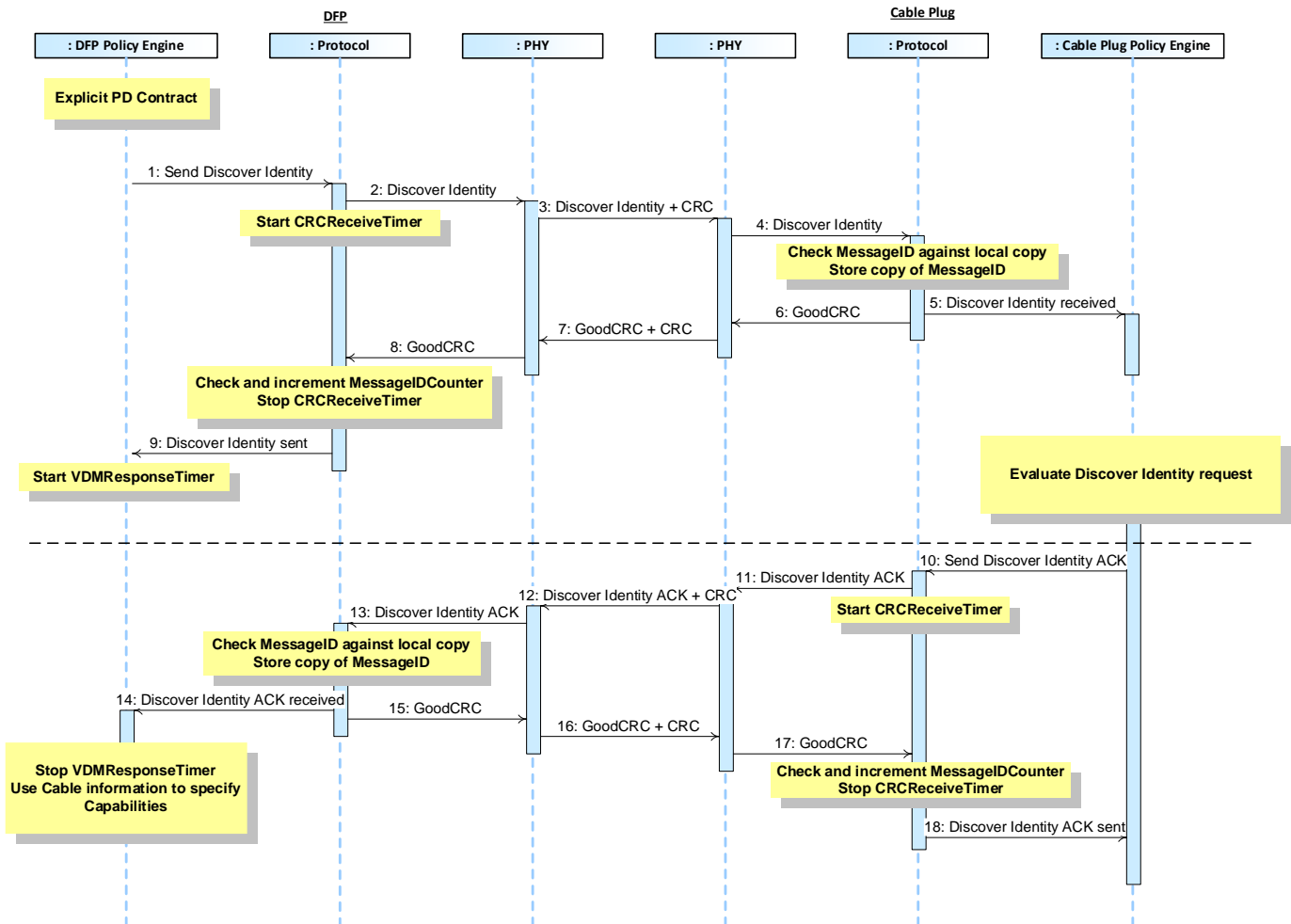
Figure 8-82 DFP to Cable Plug Discover Identity
