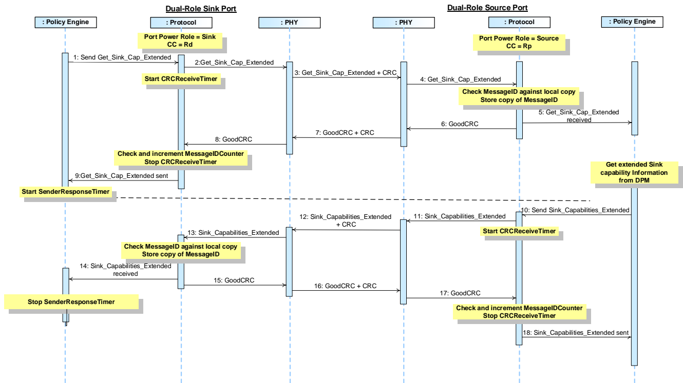
Figure 8-55 Dual-Role Sink Gets Dual-Role Source's Extended Capabilities
