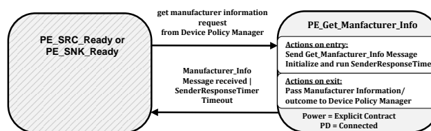
Figure 8-131 Get Manufacturer Information State Diagram
