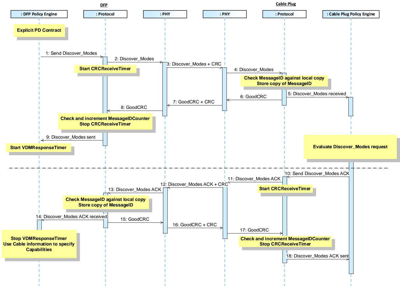
Figure 8-86 DFP to Cable Plug Discover Modes
