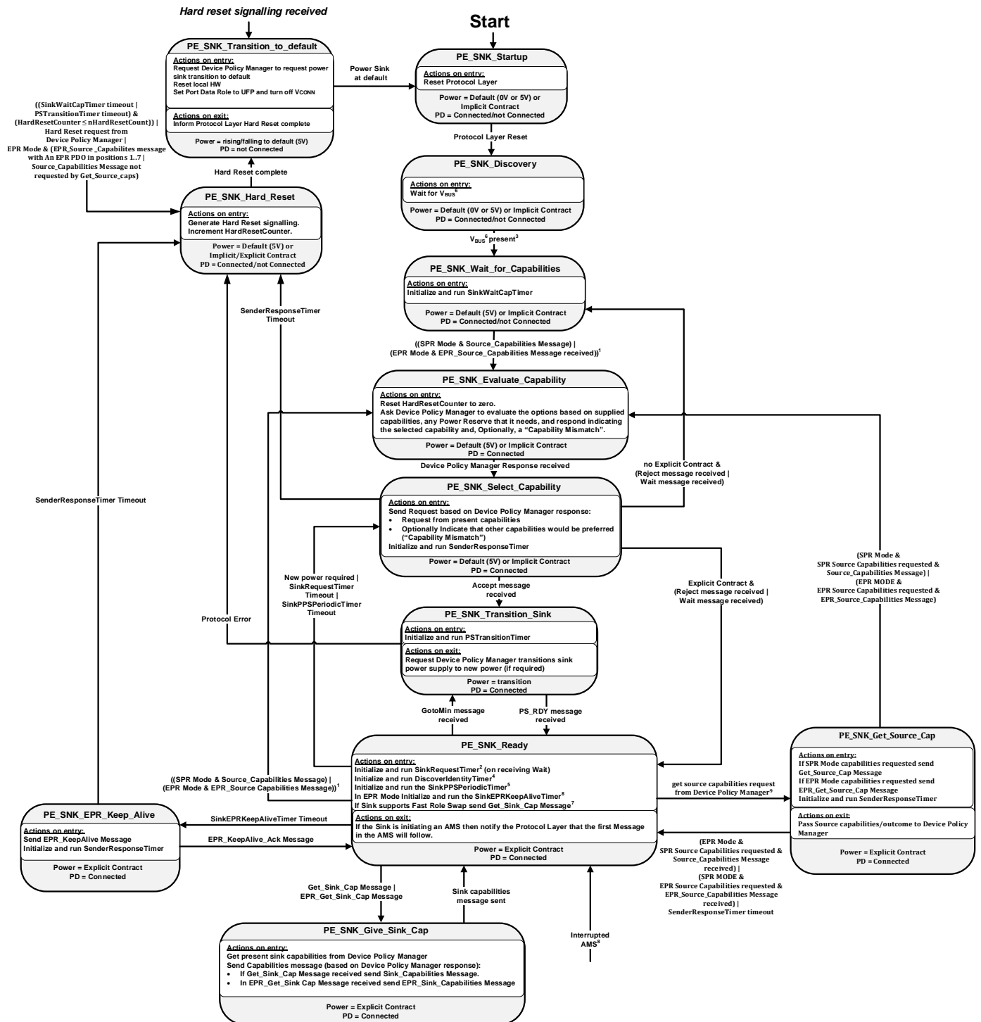
Figure 8-107 Sink Port State Diagram
