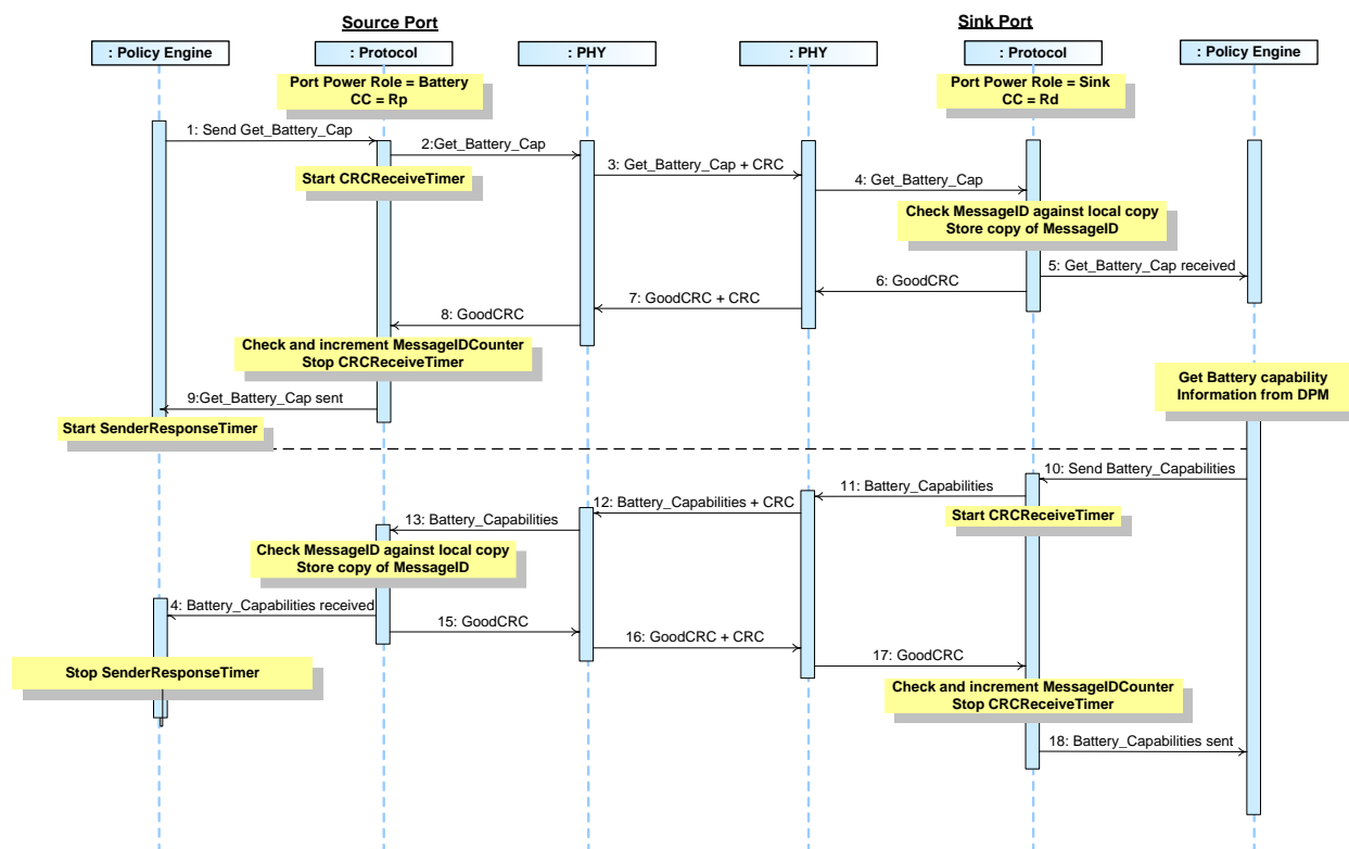
Figure 8-57 Source Gets Sink's Battery Capabilities
