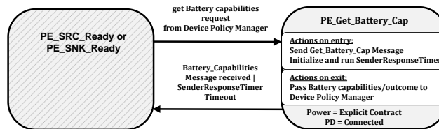
Figure 8-127 Get Battery Capabilities State Diagram
