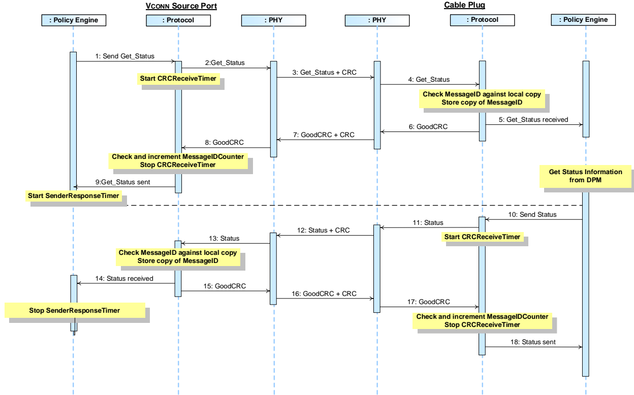
Figure 8-42 VCONN Source Gets Cable Plug Status
