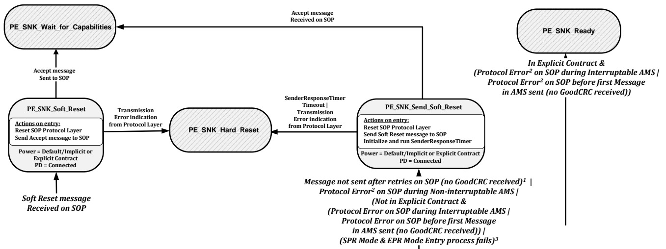
Figure 8-109 Sink Port Soft Reset and Protocol Error Diagram
