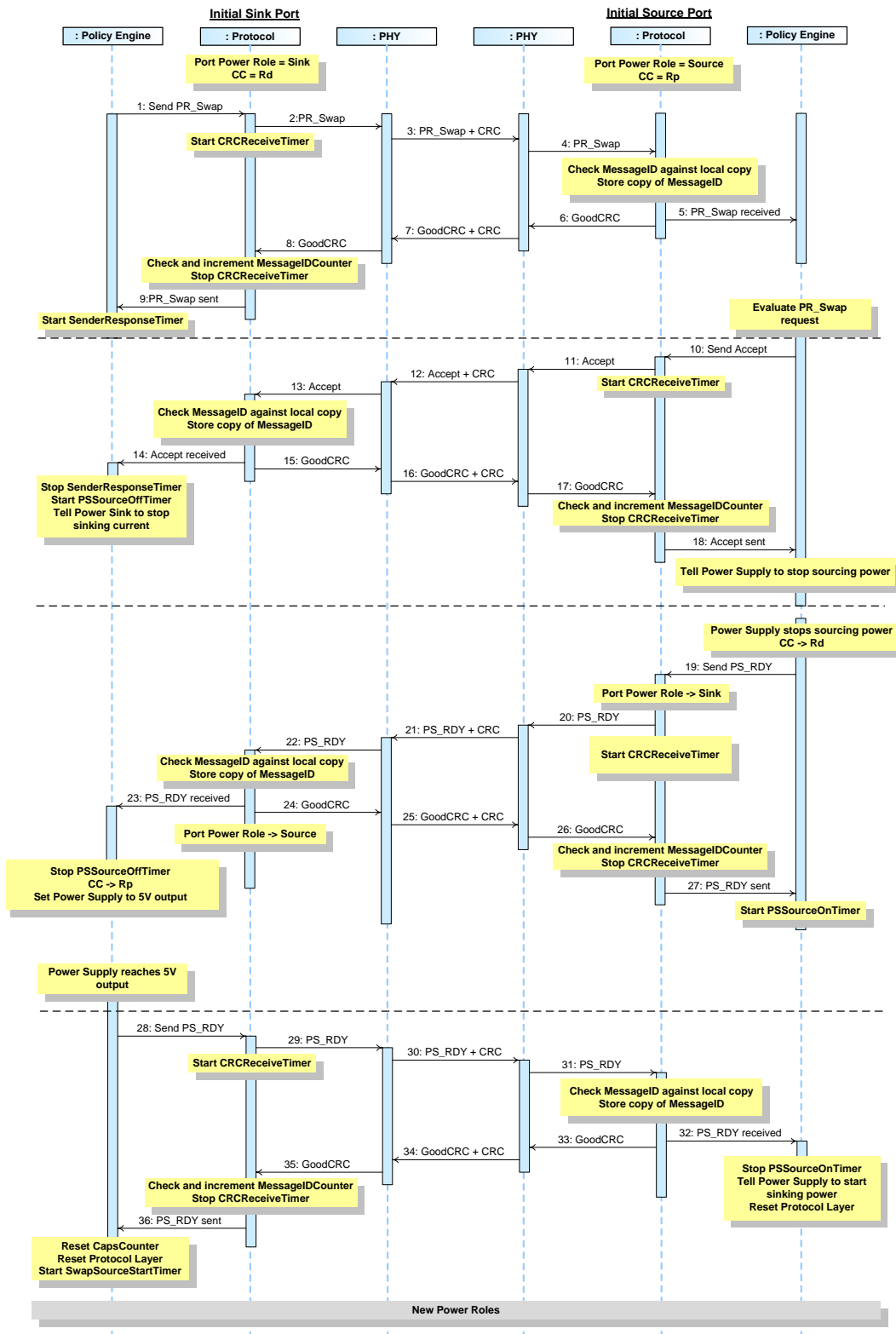
Figure 8-30 Successful Power Role Swap Sequence Initiated by the Sink
