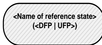
Figure 8-103 Example of state reference with conditions
