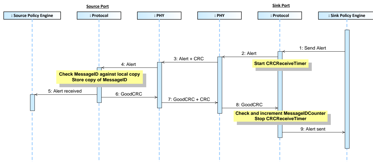
Figure 8-39 Sink Alert to Source
