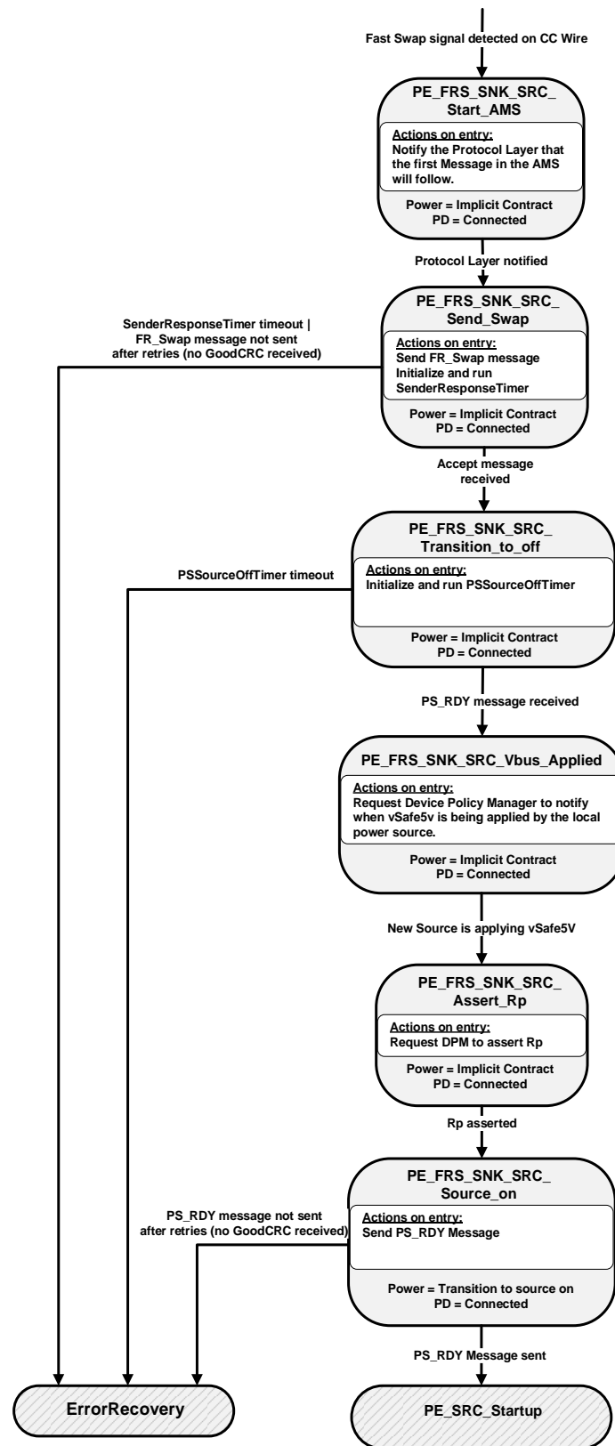
Figure 8-152: Dual-role Port in Sink to Source Fast Role Swap State Diagram
