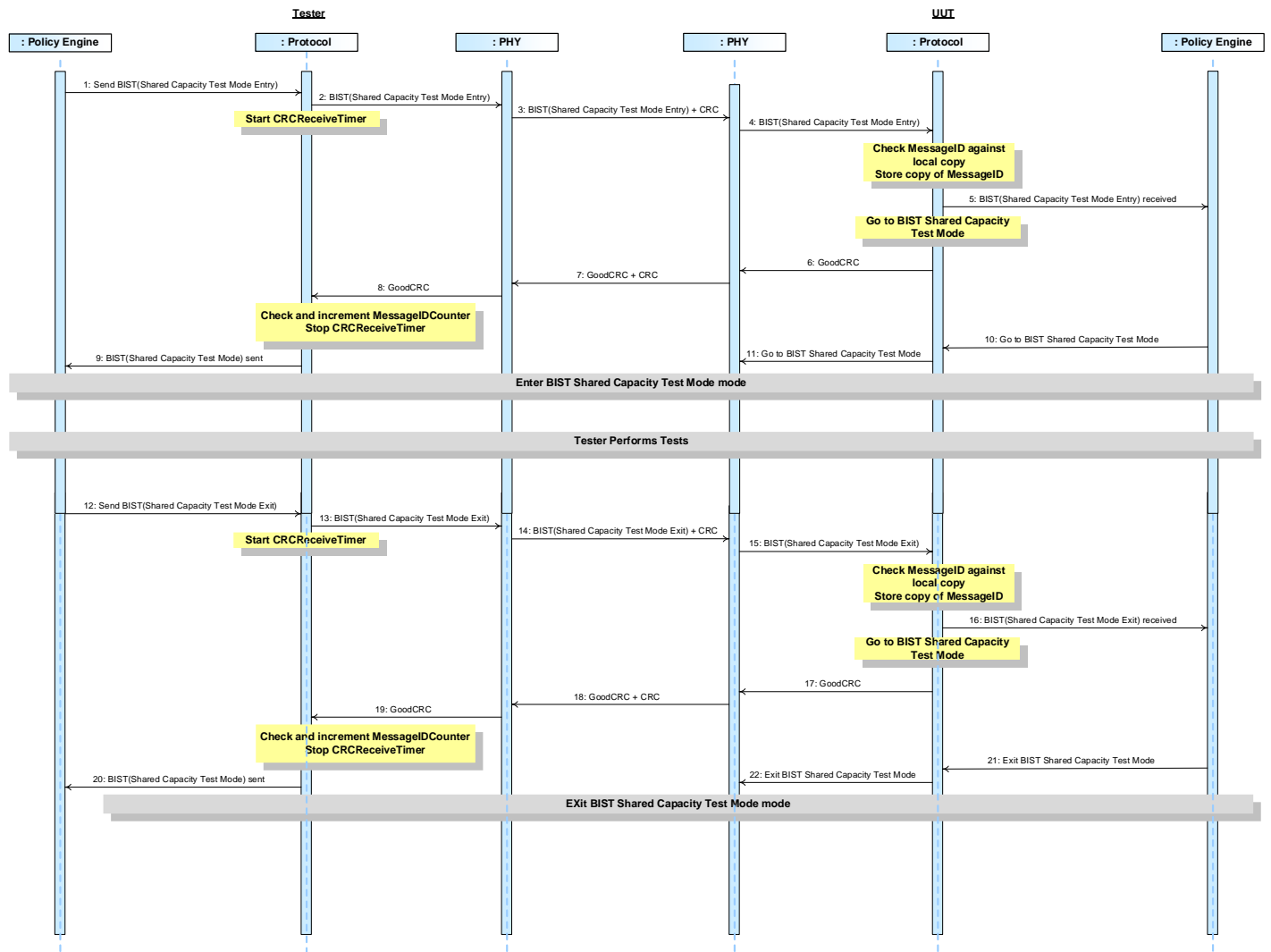
Figure 8-94 BIST Share Capacity Mode Test
