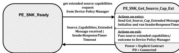
Figure 8-119 Sink Port Get Source Capabilities Extended State Diagram
