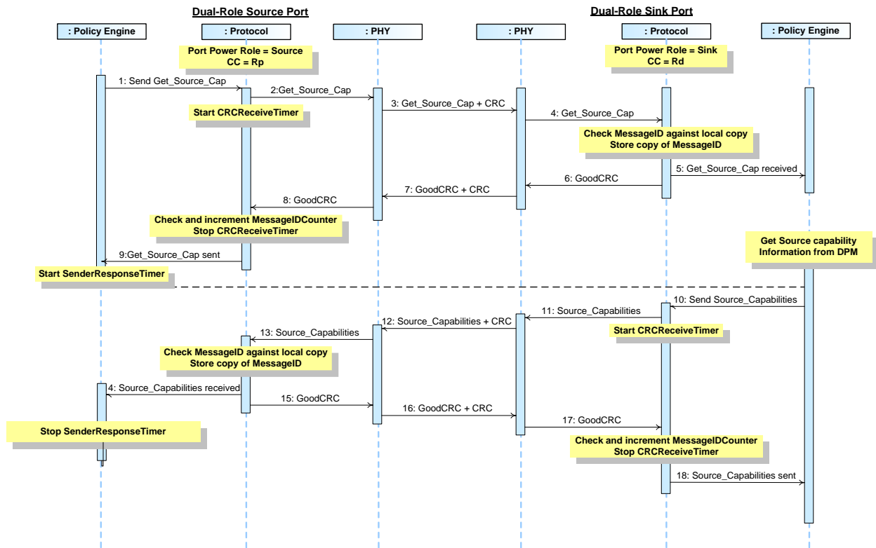
Figure 8-45 Dual-Role Source Gets Dual-Role Sink's Capabilities as a Source
