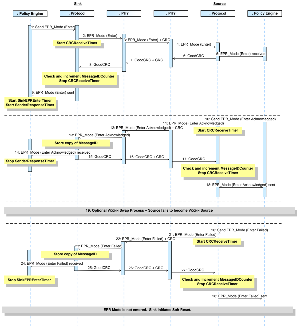
Figure 8-13 Entering EPR Mode (Failure of VCONN Swap)
