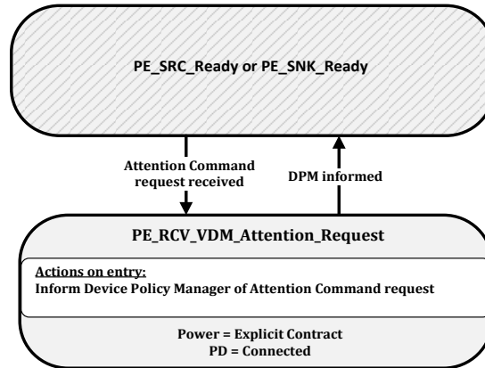
Figure 8-169 Receiving a Structured VDM Attention State Diagram
