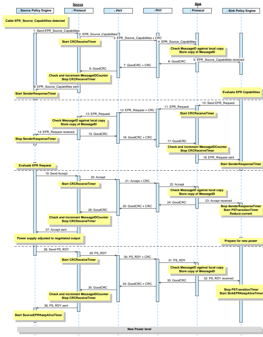
Figure 8-14 Successful Fixed EPR Power Negotiation
