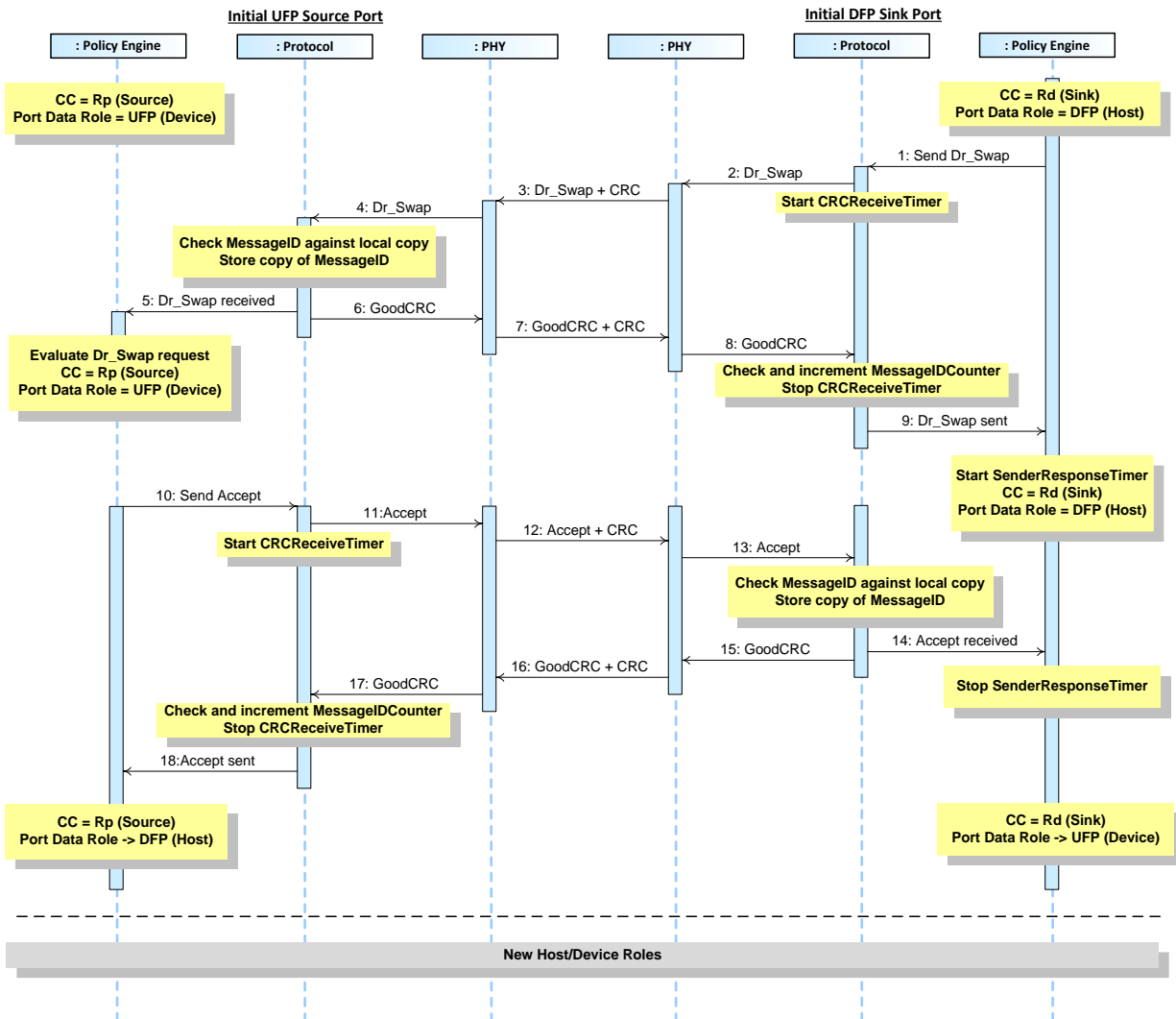
Figure 8-35 Data Role Swap, DFP operating as Sink initiates
