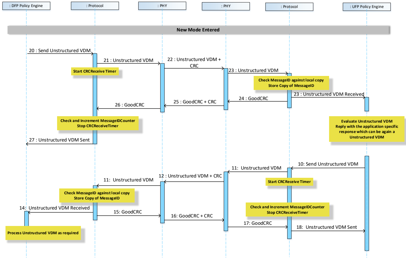
Figure 8-99 Unstructured VDM Message Sequence
