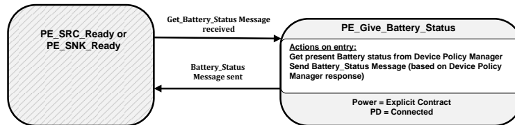
Figure 8-130 Give Battery Status State Diagram
