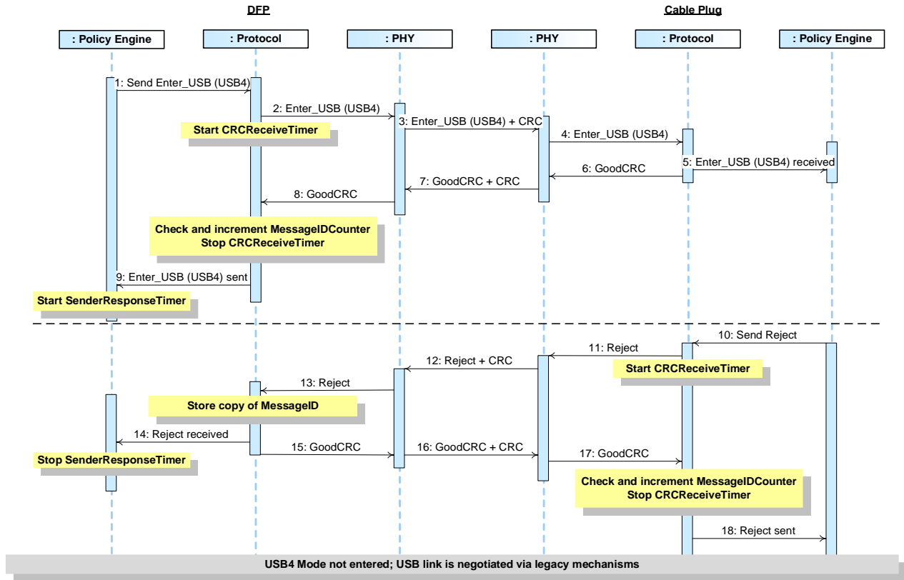
Figure 8-98 Cable Plug Entering USB4 Mode (Invalid)
