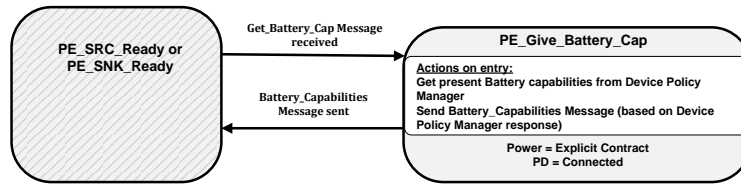
Figure 8-128 Give Battery Capabilities State Diagram
