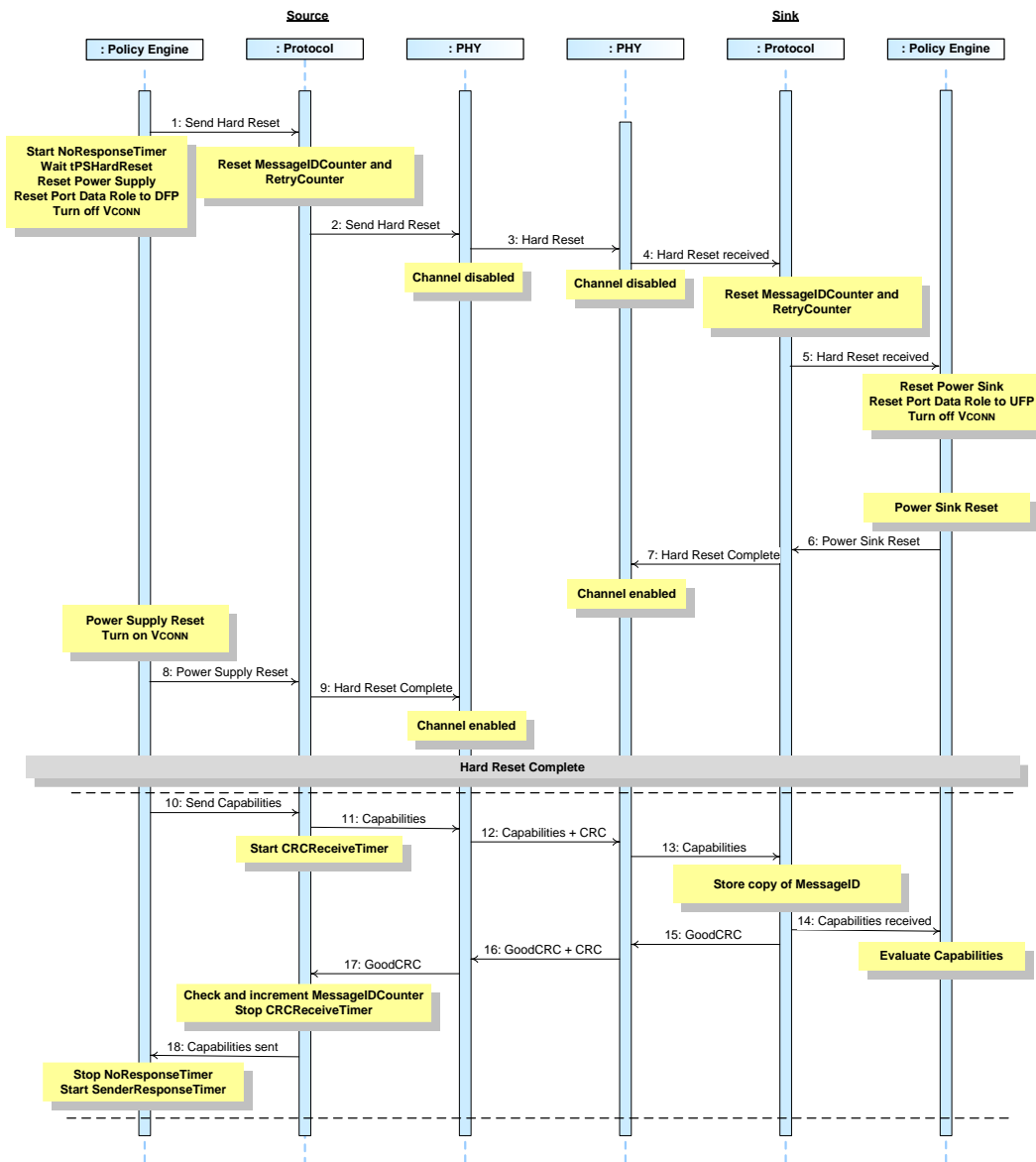
Figure 8-26 Source initiated Hard Reset
