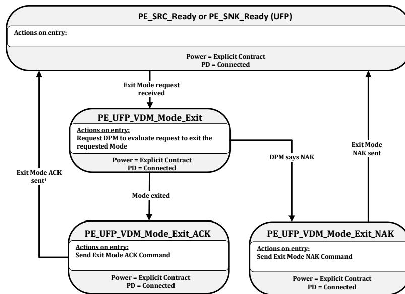
Figure 8-173 UFP Structured VDM Exit Mode State Diagram
