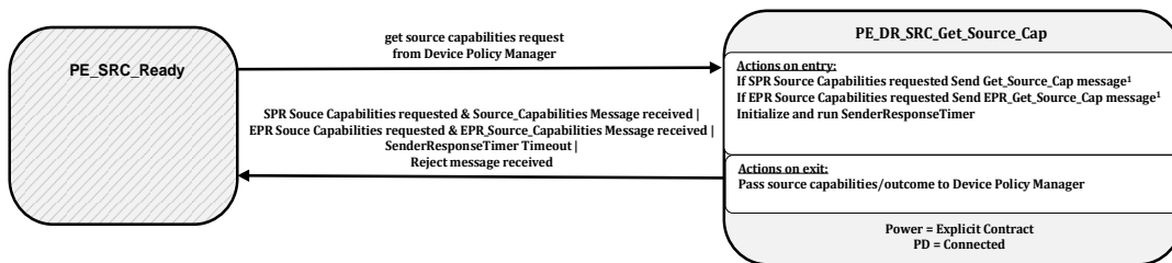
Figure 8-153 Dual-Role (Source) Get Source Capabilities diagram
