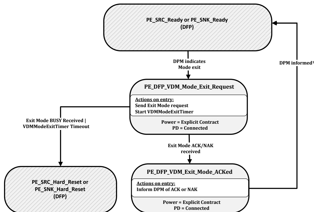
Figure 8-171 DFP VDM Mode Exit State Diagram
