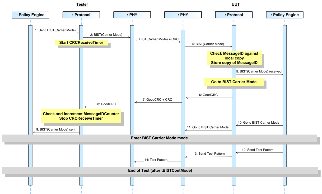
Figure 8-92 BIST Carrier Mode Test
