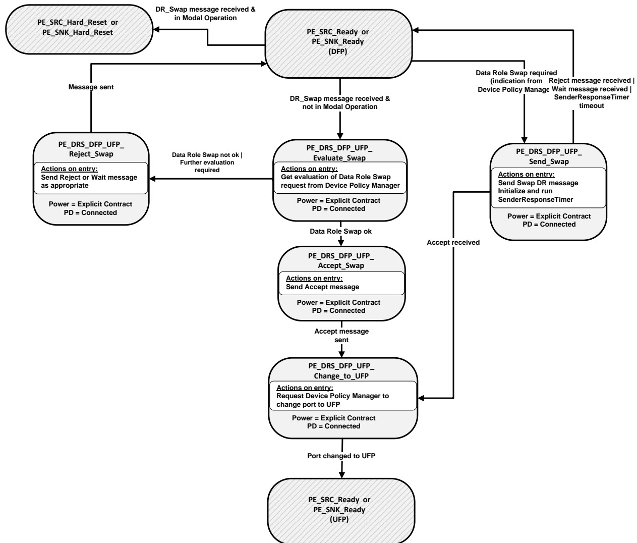
Figure 8-147: DFP to UFP Data Role Swap State Diagram
