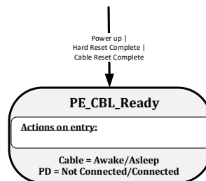
Figure 8-174 Cable Ready VDM State Diagram
