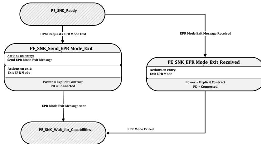
Figure 8-185 Sink EPR Mode Exit State Diagram
