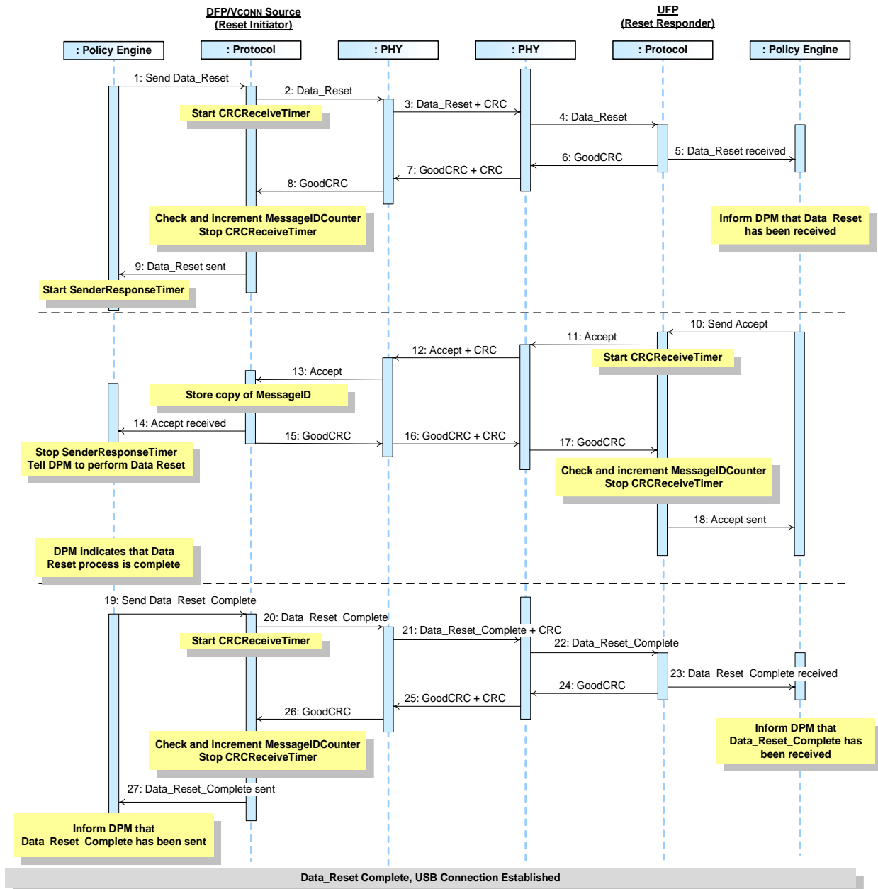
Figure 8-22 DFP Initiated Data Reset where the DFP is the VCONN Source
