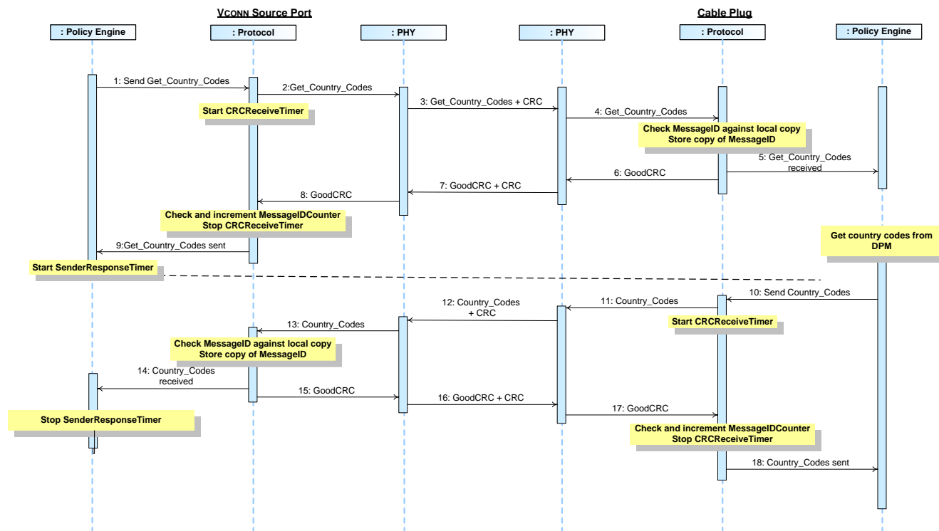
Figure 8-67 VCONN Source Gets Cable Plug's Country Codes
