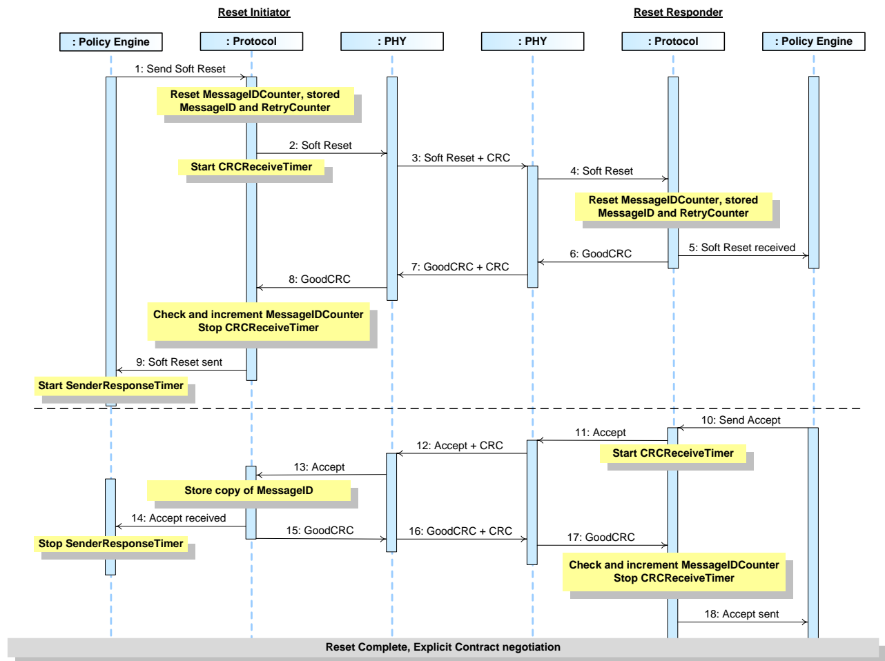
Figure 8-21 Soft Reset
