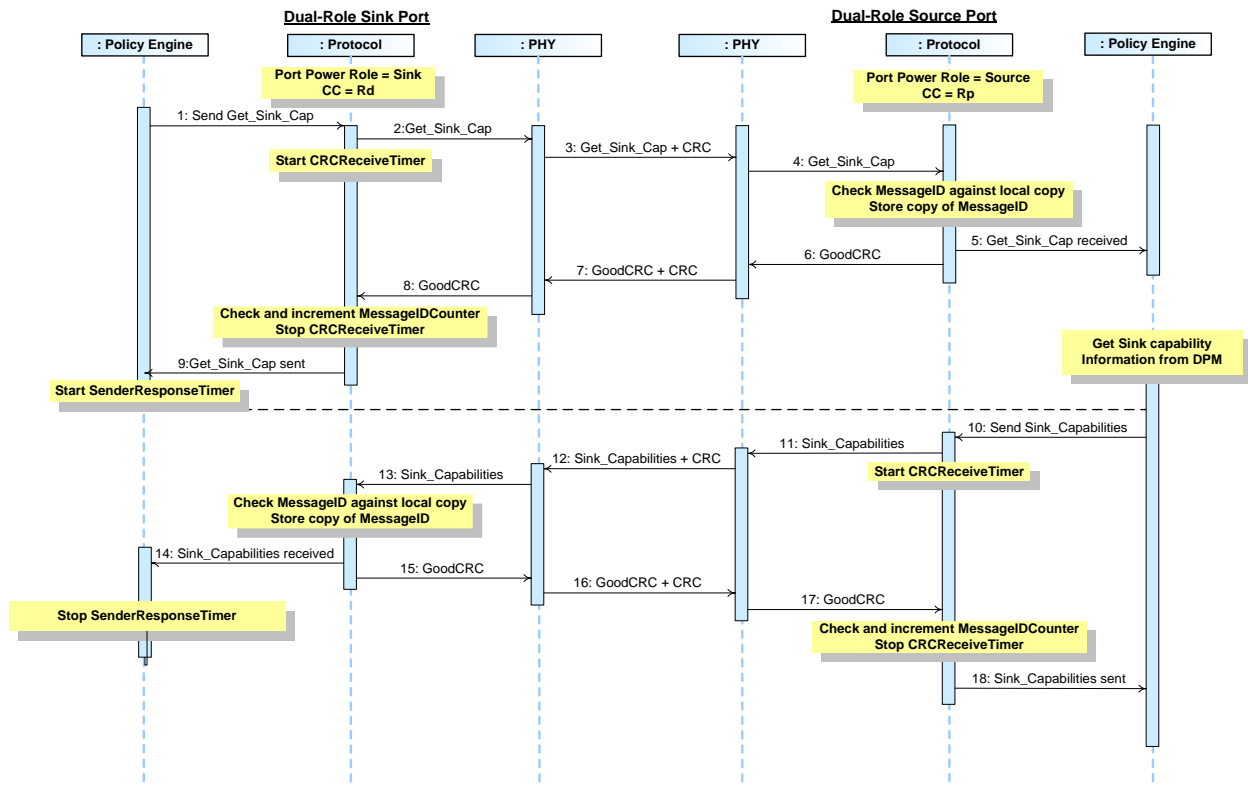
Figure 8-47 Dual-Role Sink Gets Dual-Role Source's Capabilities as a Sink
