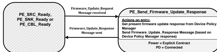
Figure 8-145 Send firmware update response State Diagram
