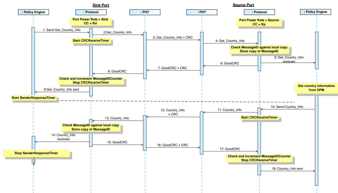
Figure 8-72 Sink Gets Source's Revision Information
