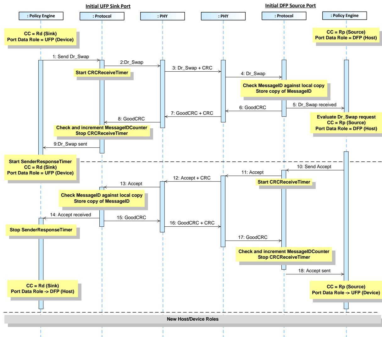
Figure 8-32 Data Role Swap, UFP operating as Sink initiates
