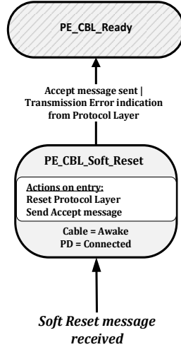
Figure 8-175 Cable Plug Soft Reset State Diagram
