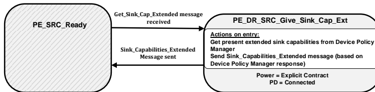
Figure 8-160 Dual-Role (Source) Give Sink Capabilities diagram
