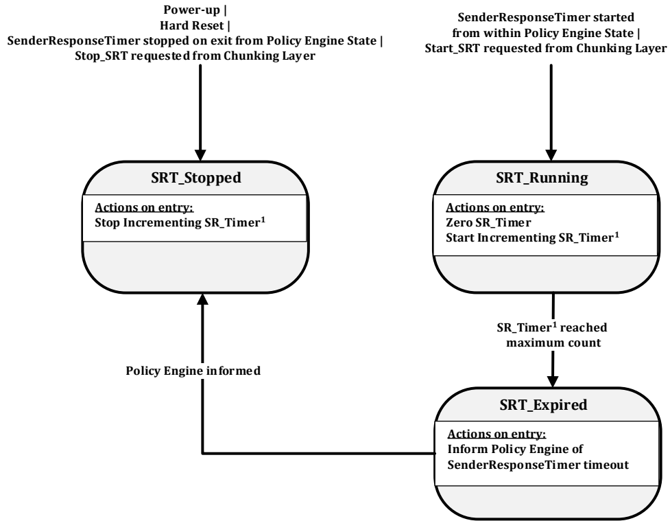
Figure 8-105 SenderResponseTimer Policy Engine State Diagram
