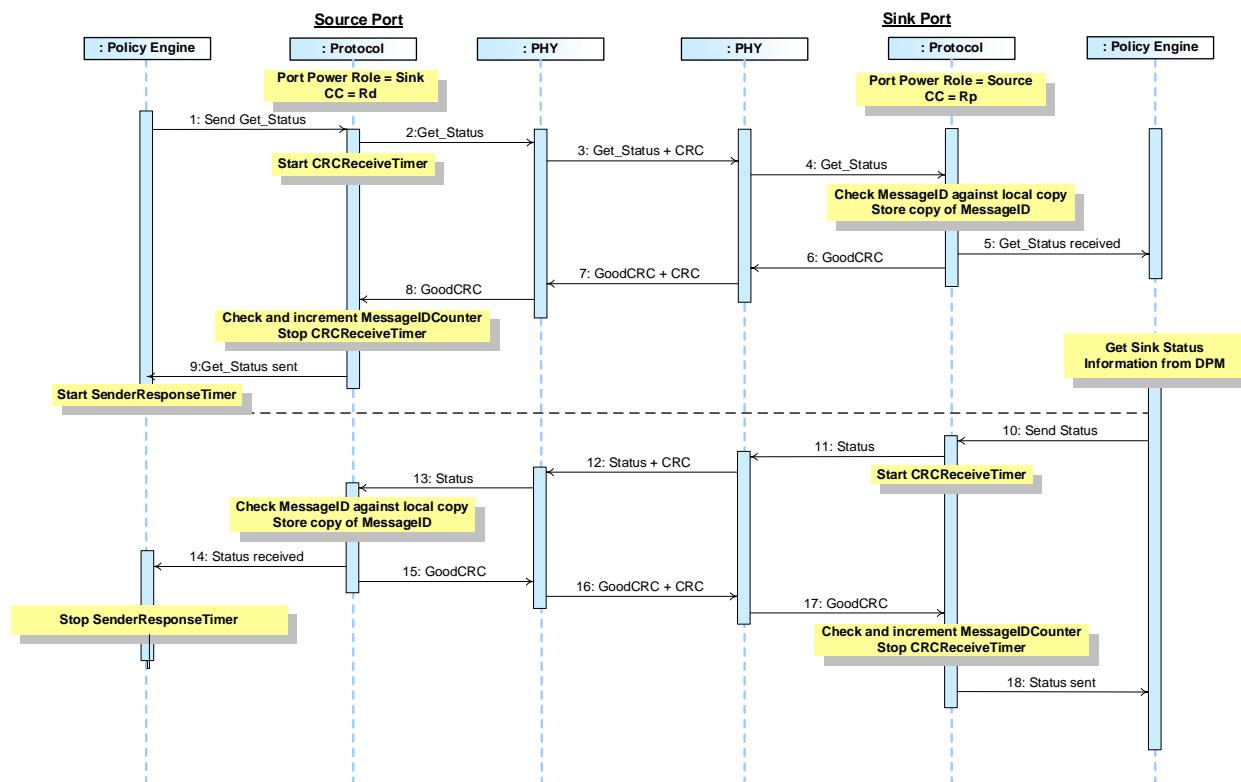
Figure 8-41 Source Gets Sink Status
