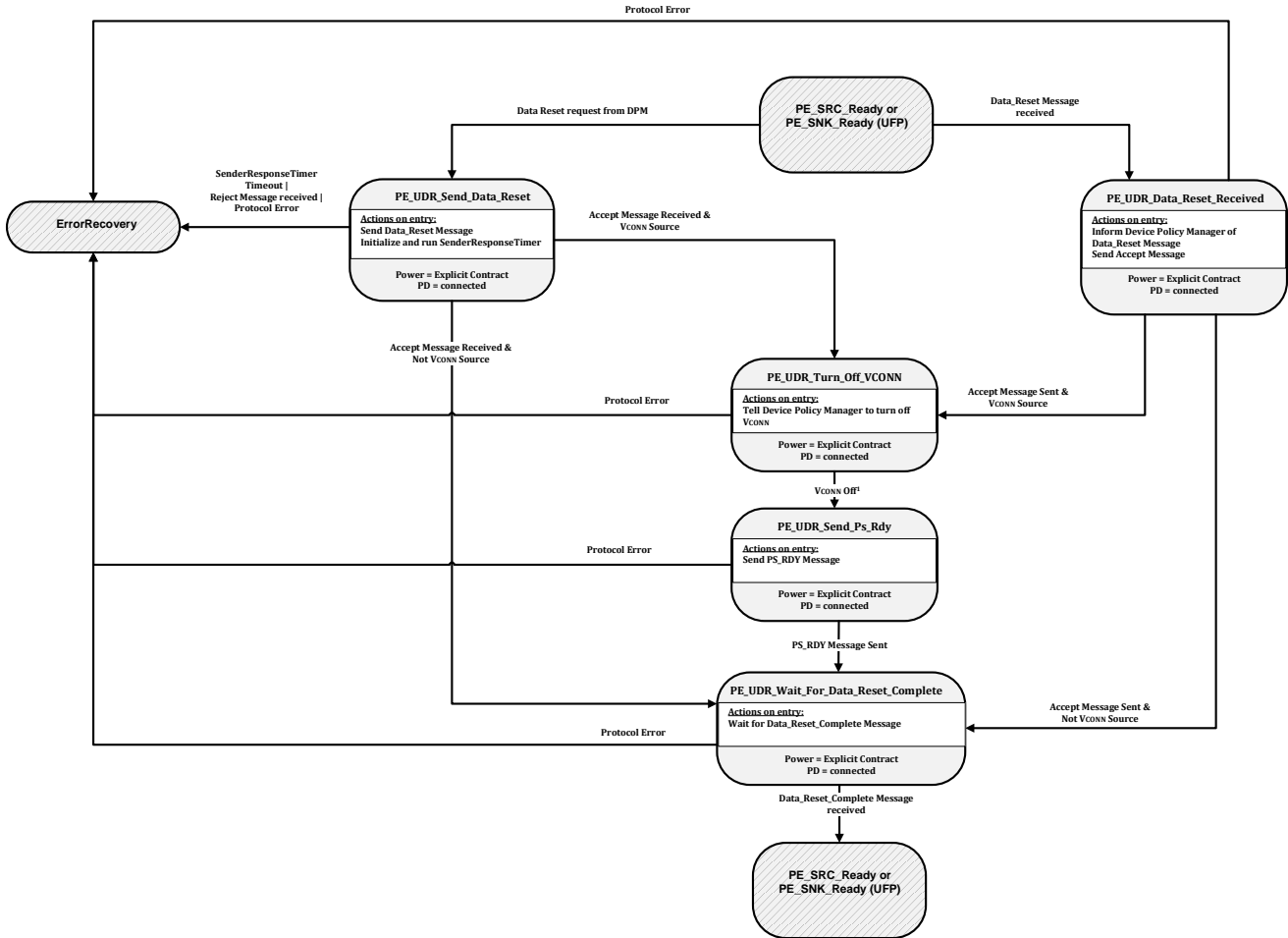
Figure 8-111 UFP Data_Reset Message State Diagram
