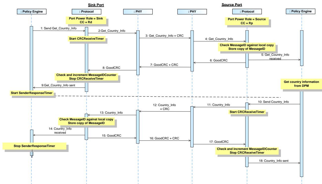
Figure 8-69 Sink Gets Source's Country Information
