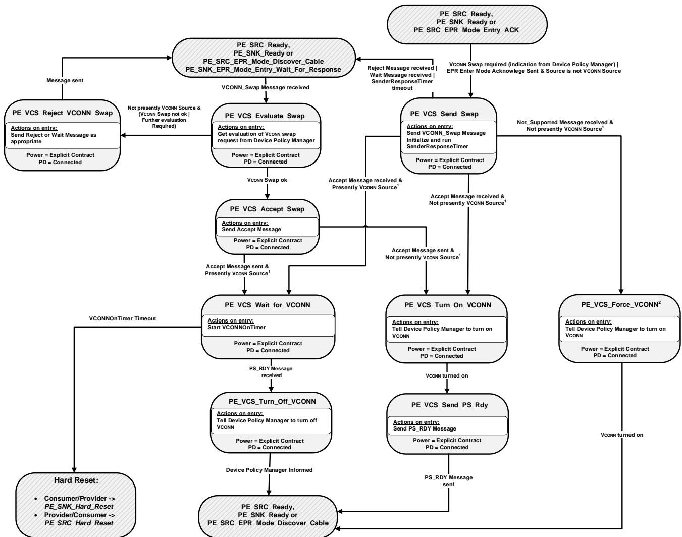
Figure 8-161 VCONN Swap State Diagram
