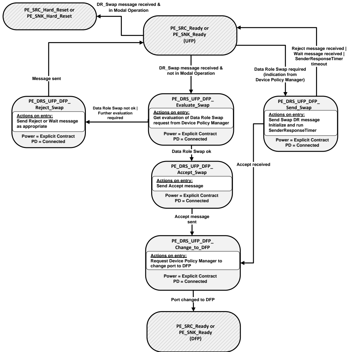
Figure 8-148: UFP to DFP Data Role Swap State Diagram
