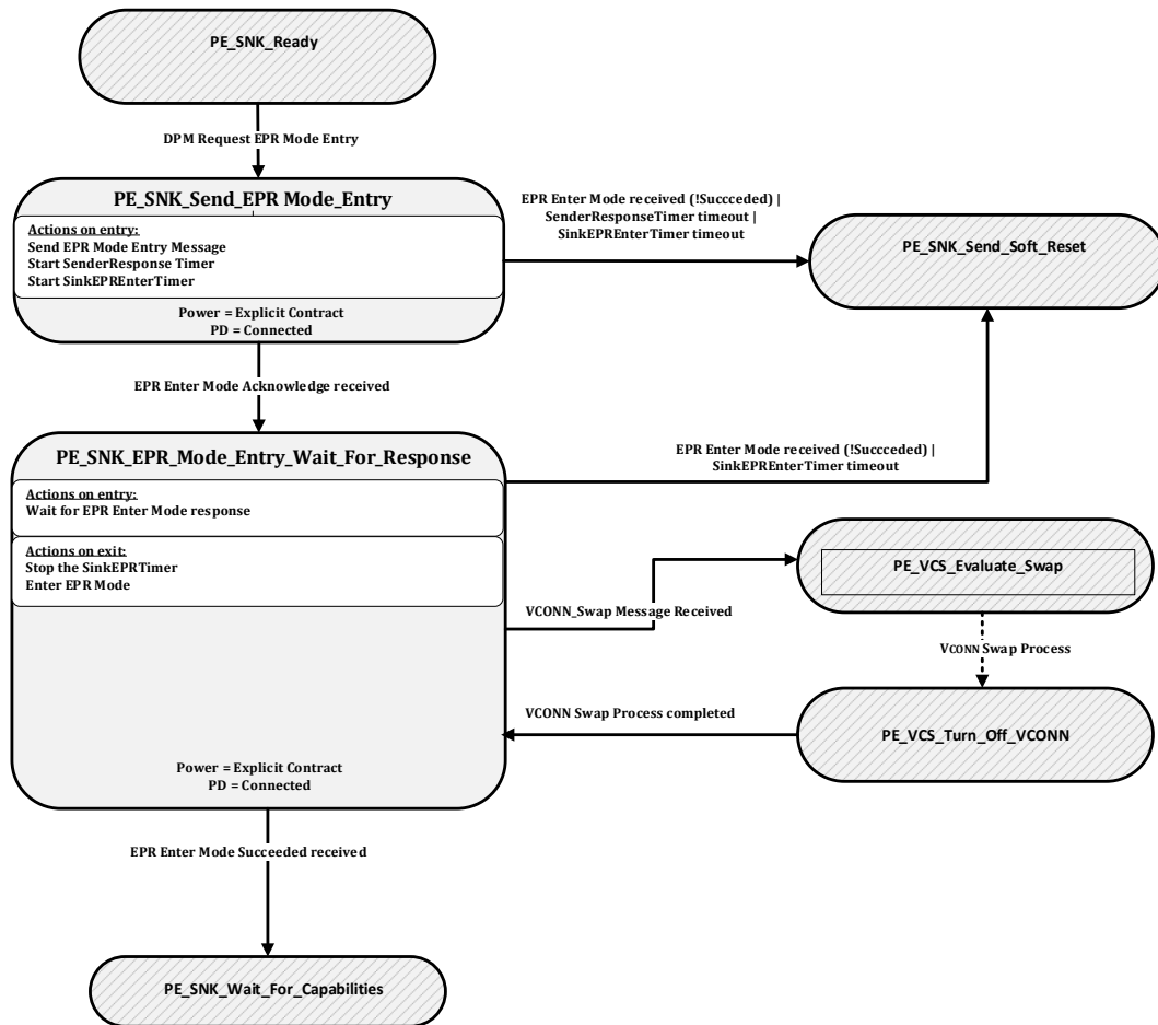
Figure 8-183 Sink EPR Mode Entry State Diagram
