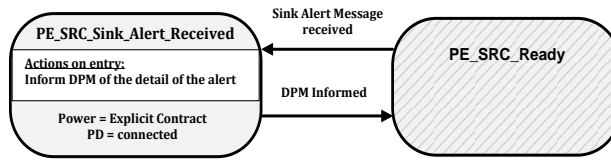
Figure 8-118 Source Port Sink Alert State Diagram
