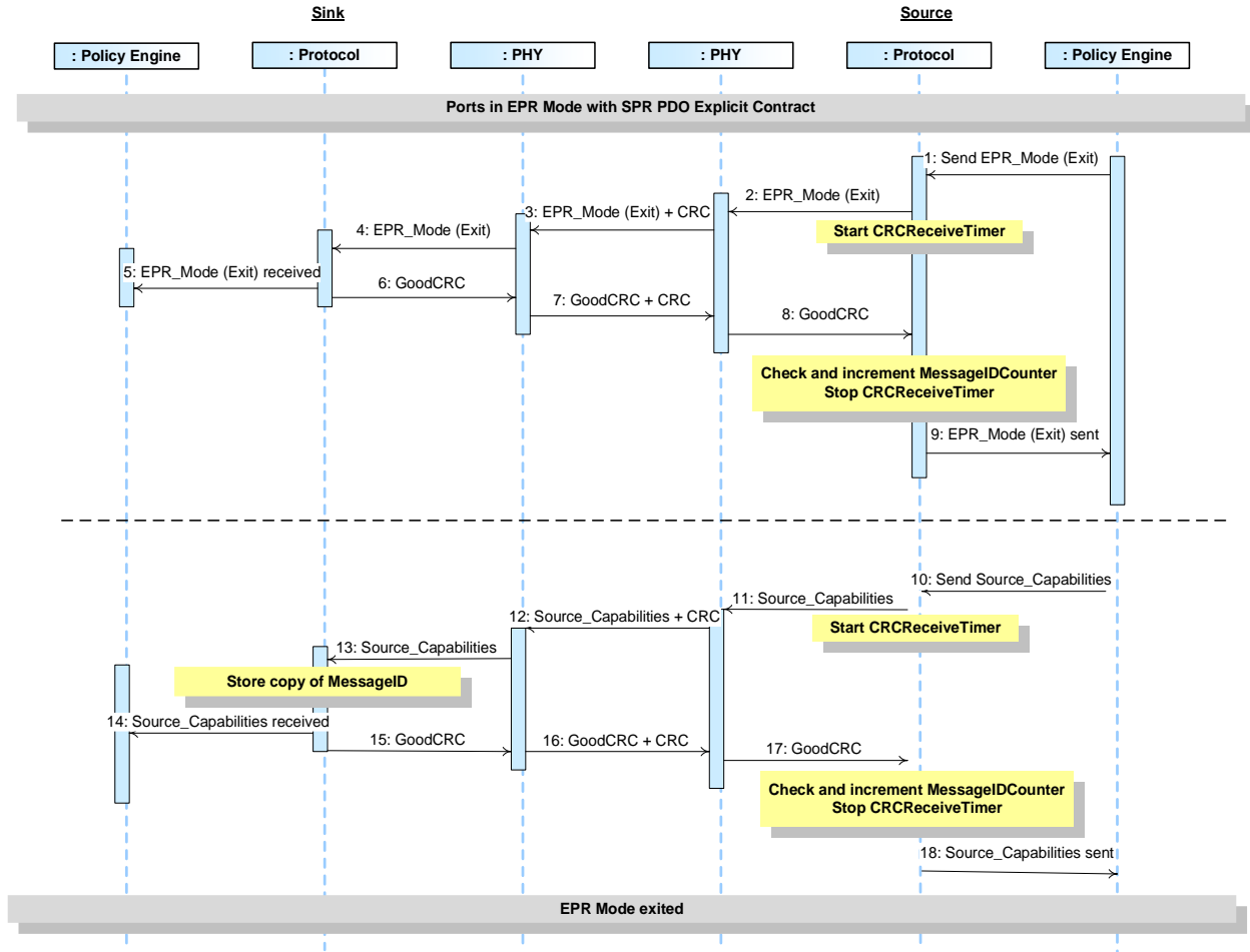
Figure 8-17 Exiting EPR Mode (Source Initiated)
