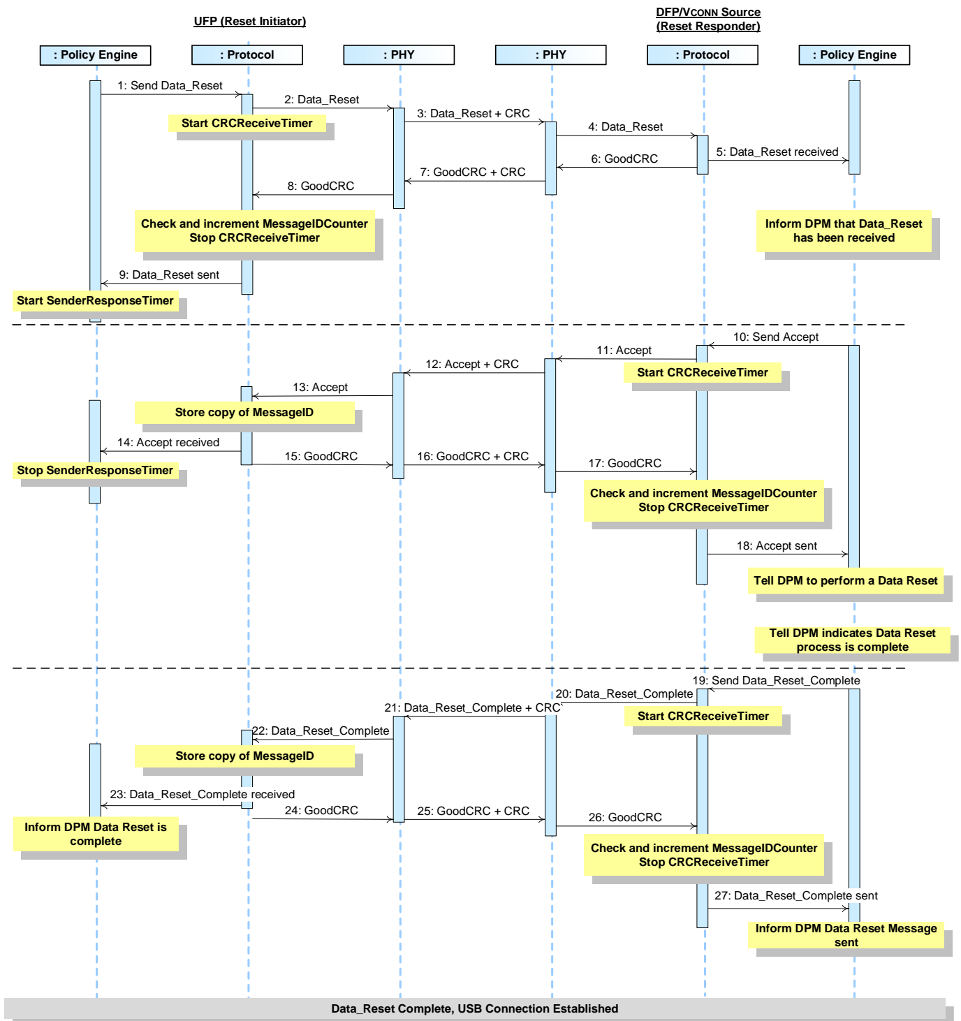
Figure 8-23 DFP Receives Data Reset where the DFP is the VCONN Source
