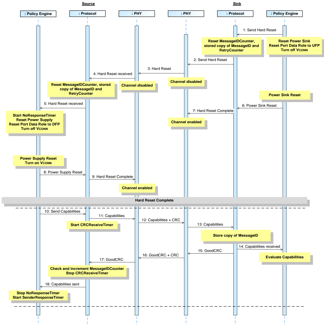
Figure 8-27 Sink Initiated Hard Reset
