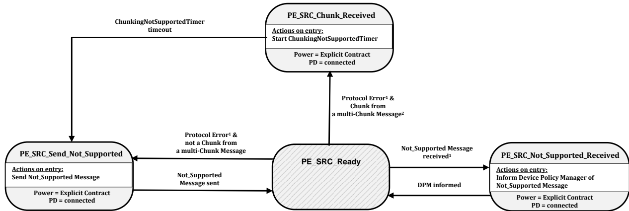
Figure 8-112 Source Port Not Supported Message State Diagram
