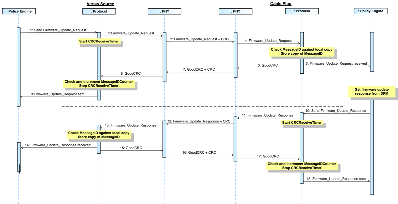
Figure 8-79 VCONN Source requests firmware update exchange with Cable Plug
