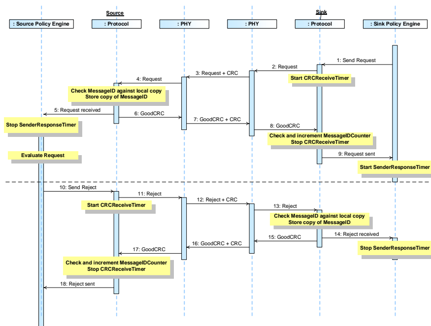
Figure 8-9 SPR Sink Makes Request (Reject)
