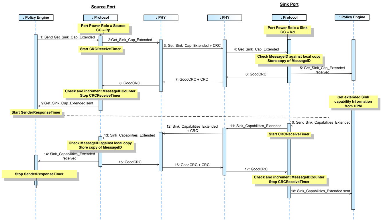
Figure 8-54 Source Gets Sink's Extended Capabilities
