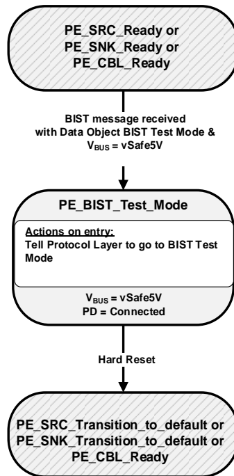
Figure 8-187 BIST Test Mode State Diagram
