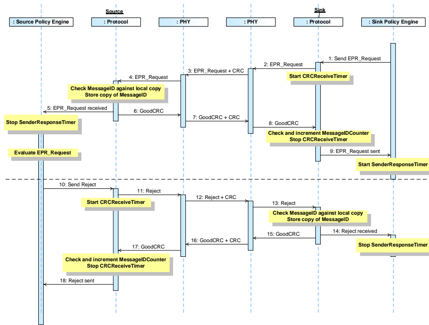
Figure 8-19 SPR Sink Makes Request (Reject)
