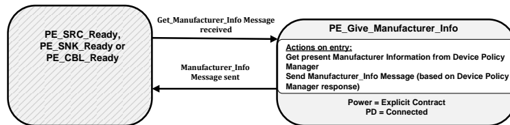
Figure 8-132 Give Manufacturer Information State Diagram
