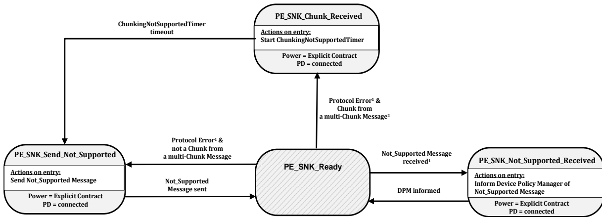
Figure 8-113 Sink Port Not Supported Message State Diagram
