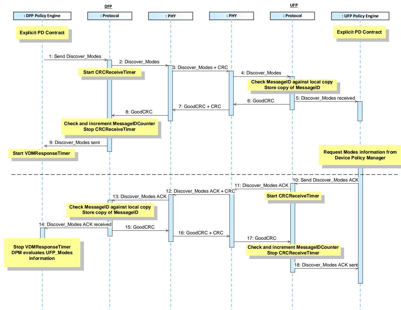
Figure 8-85 DFP to UFP Discover Modes
