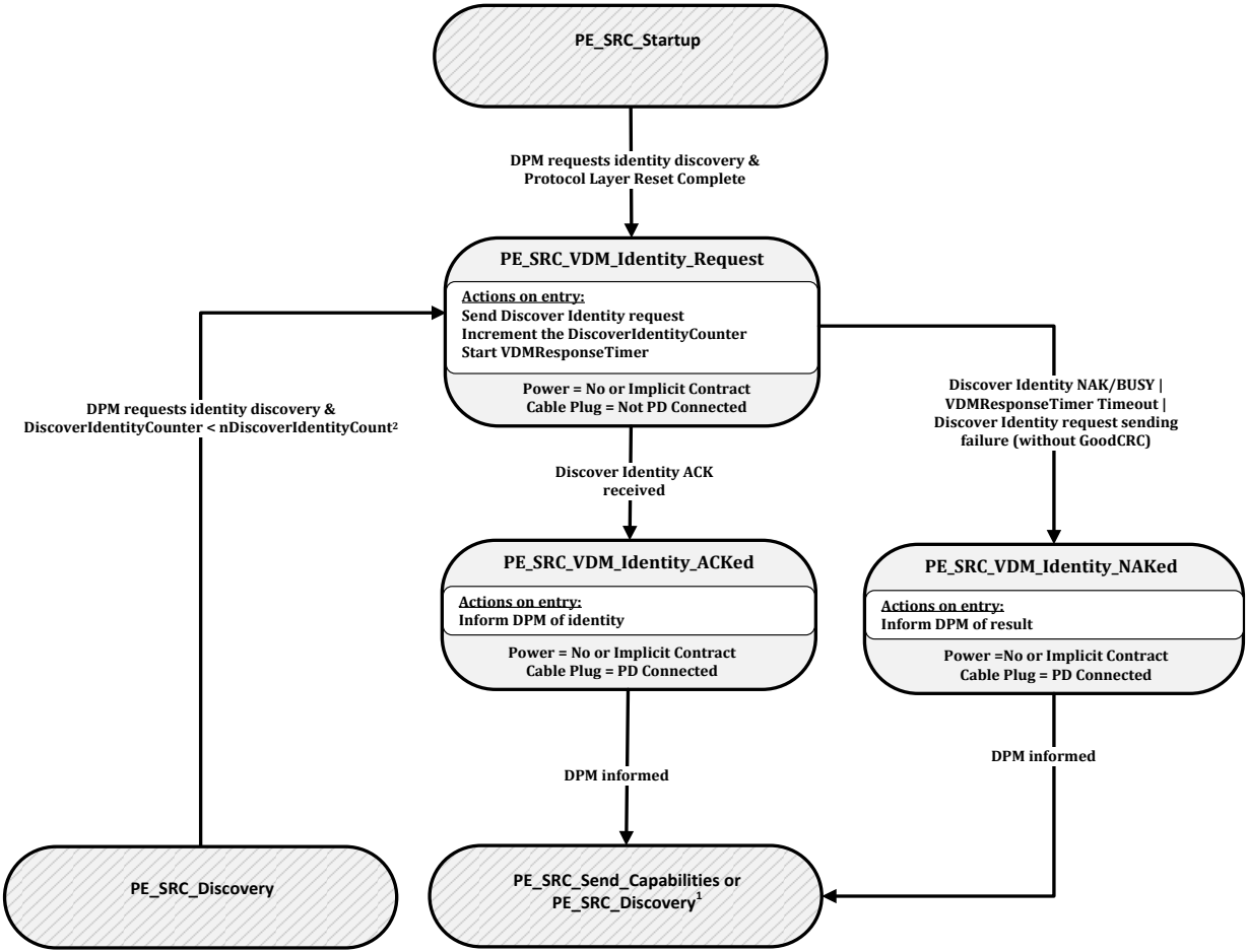
Figure 8-179 Source Startup Structured VDM Discover Identity State Diagram
