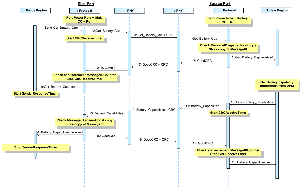
Figure 8-56 Sink Gets Source's Battery Capabilities
