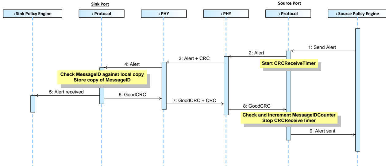
Figure 8-38 Source Alert to Sink
