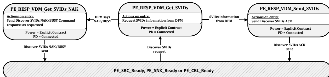
Figure 8-167 Responder Structured VDM Discover SVIDs State Diagram
