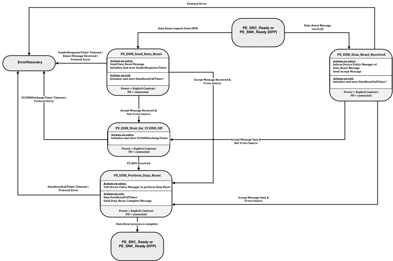
Figure 8-110 DFP Data_Reset Message State Diagram
