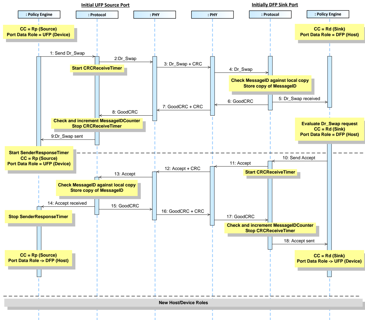
Figure 8-33 Data Role Swap, UFP operating as Source initiates
