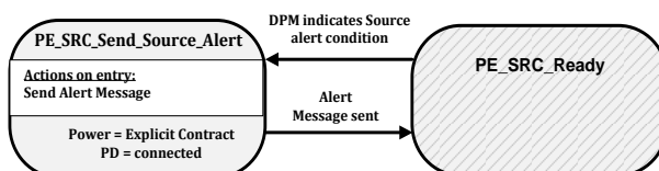
Figure 8-115 Source Port Source Alert State Diagram
