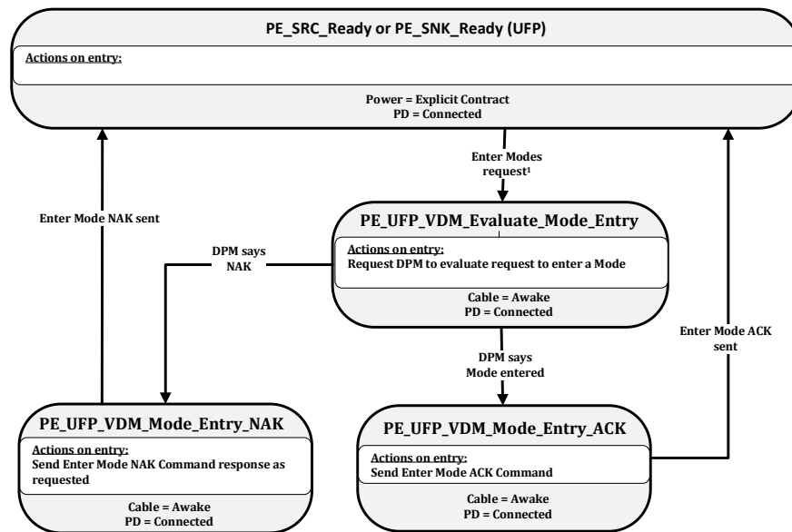
Figure 8-172 UFP Structured VDM Enter Mode State Diagram
