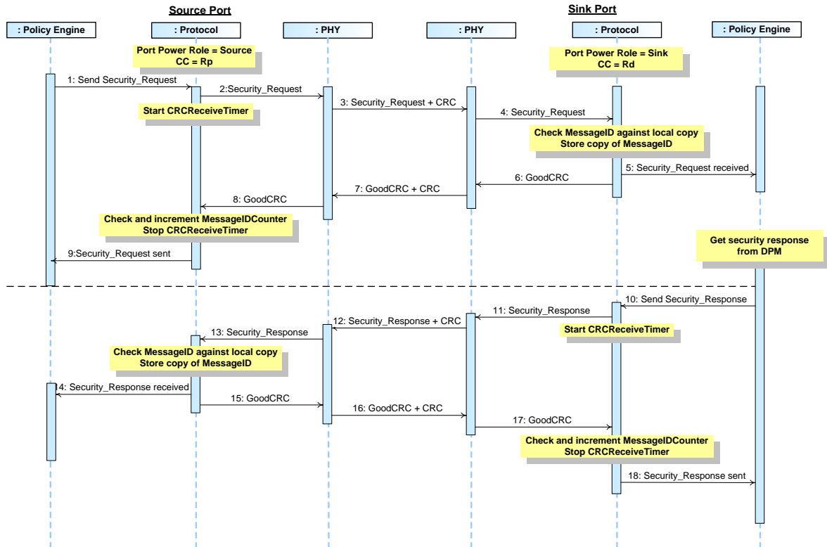
Figure 8-74 Source requests security exchange with Sink
