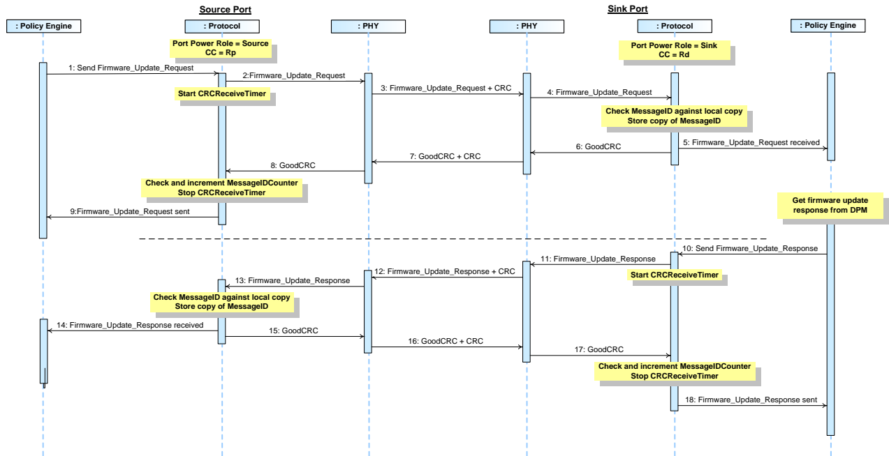
Figure 8-77 Source requests firmware update exchange with Sink
