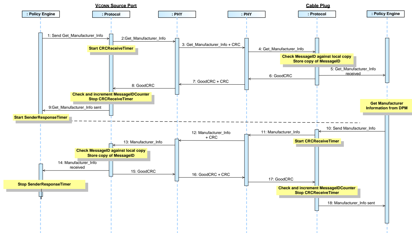
Figure 8-64 VCONN Source Gets Cable Plug's Manufacturer Information
