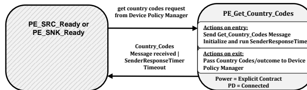
Figure 8-133 Get Country Codes State Diagram
