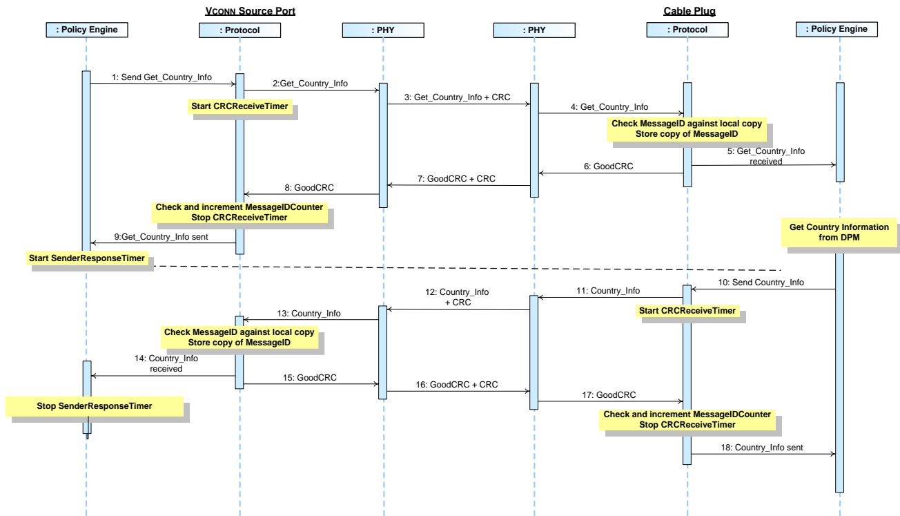
Figure 8-70 VCONN Source Gets Cable Plug's Country Information
