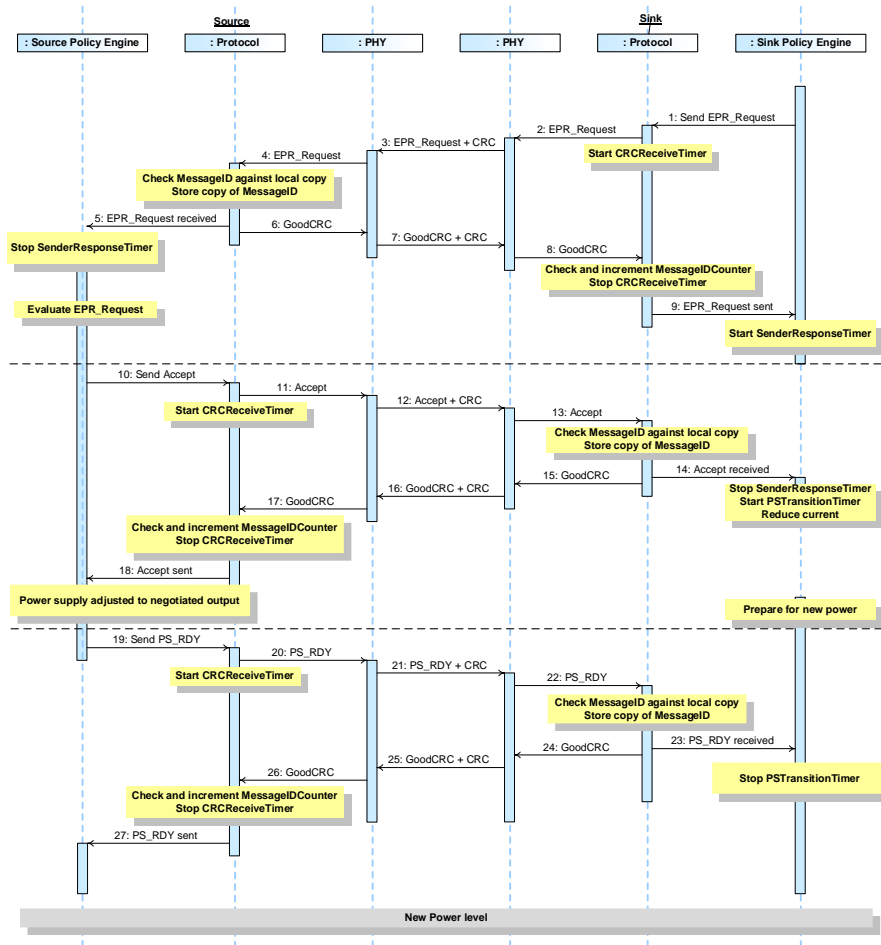
Figure 8-18 EPR Sink Makes Request (Accept)
