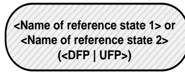
Figure 8-104 Example of state reference with the same entry and exit
