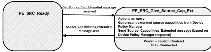
Figure 8-120 Source Give Source Capabilities Extended State Diagram
