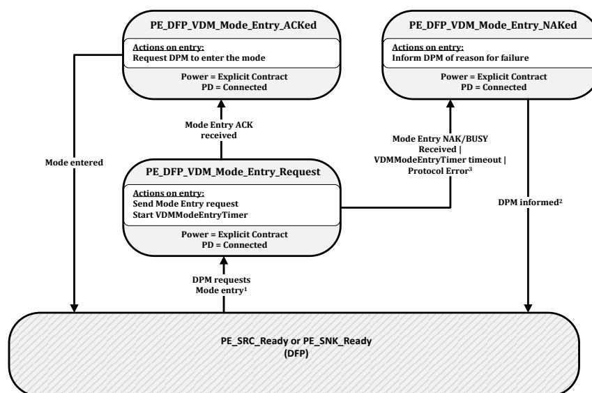
Figure 8-170 DFP VDM Mode Entry State Diagram
