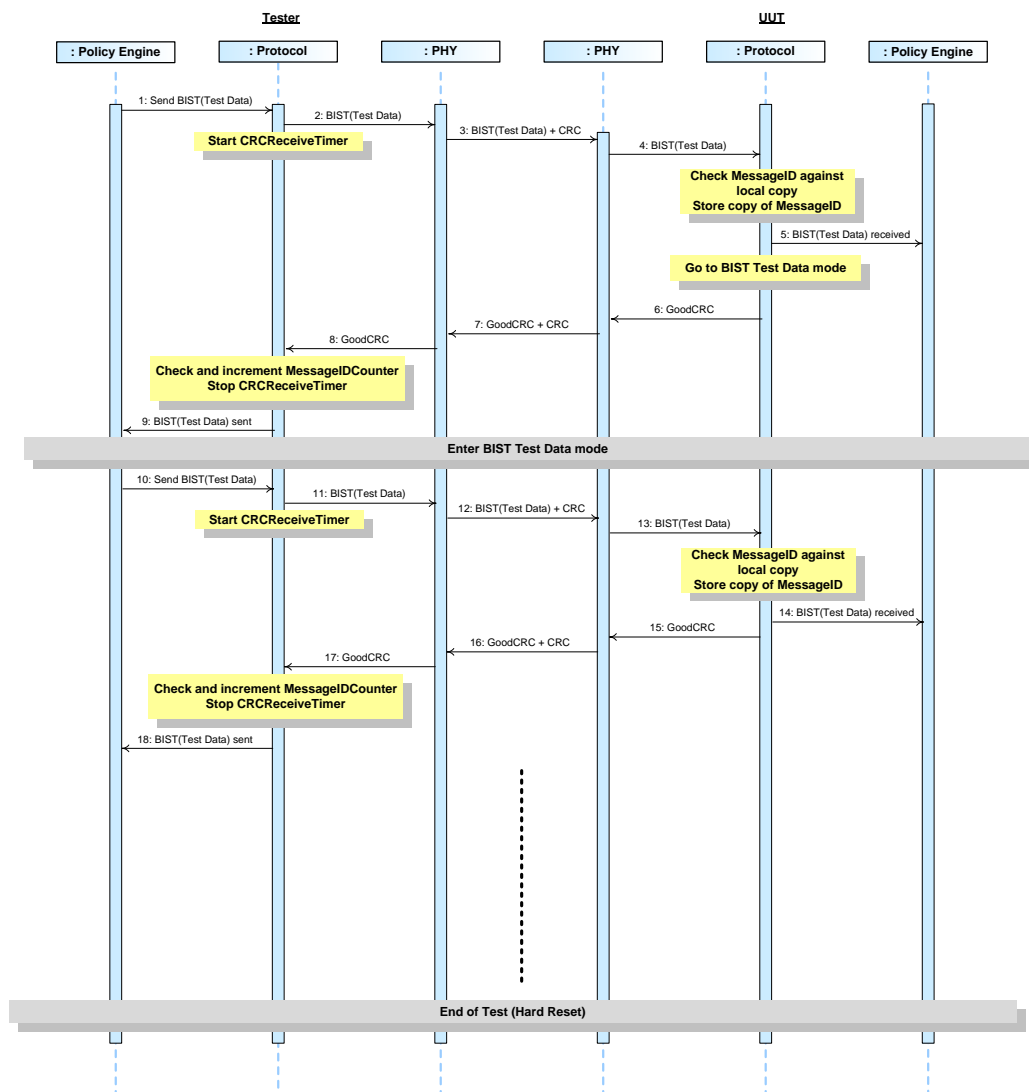
Figure 8-93 BIST Test Data Test
