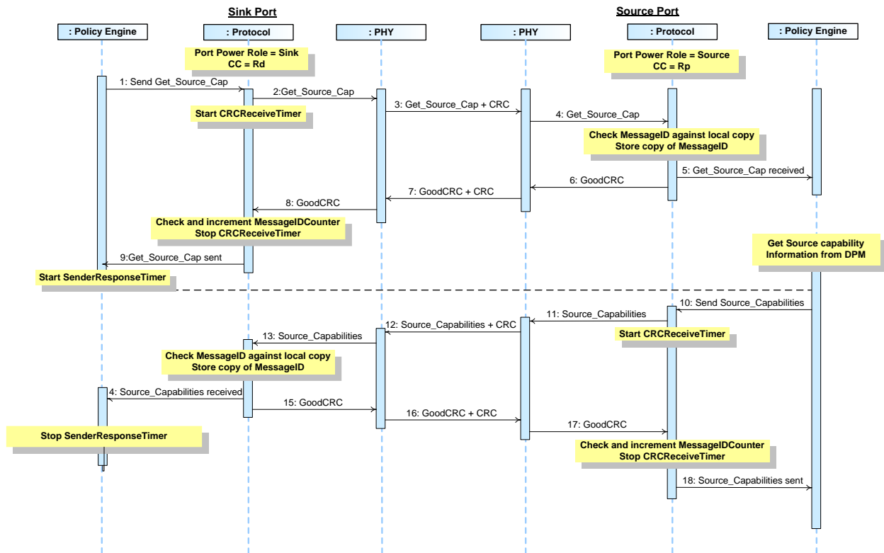
Figure 8-44 Sink Gets Source's Capabilities
