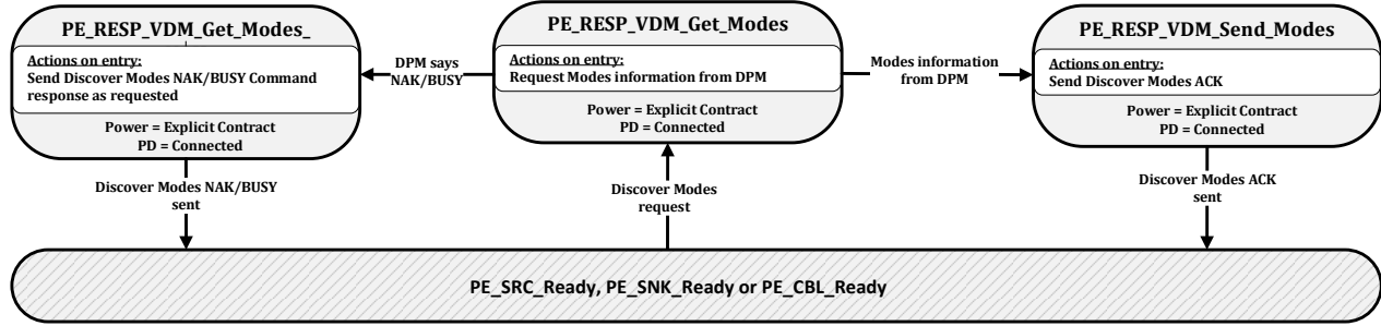
Figure 8-168 Responder Structured VDM Discover Modes State Diagram
