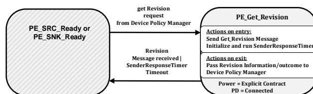
Figure 8-137 Get Revision State Diagram
