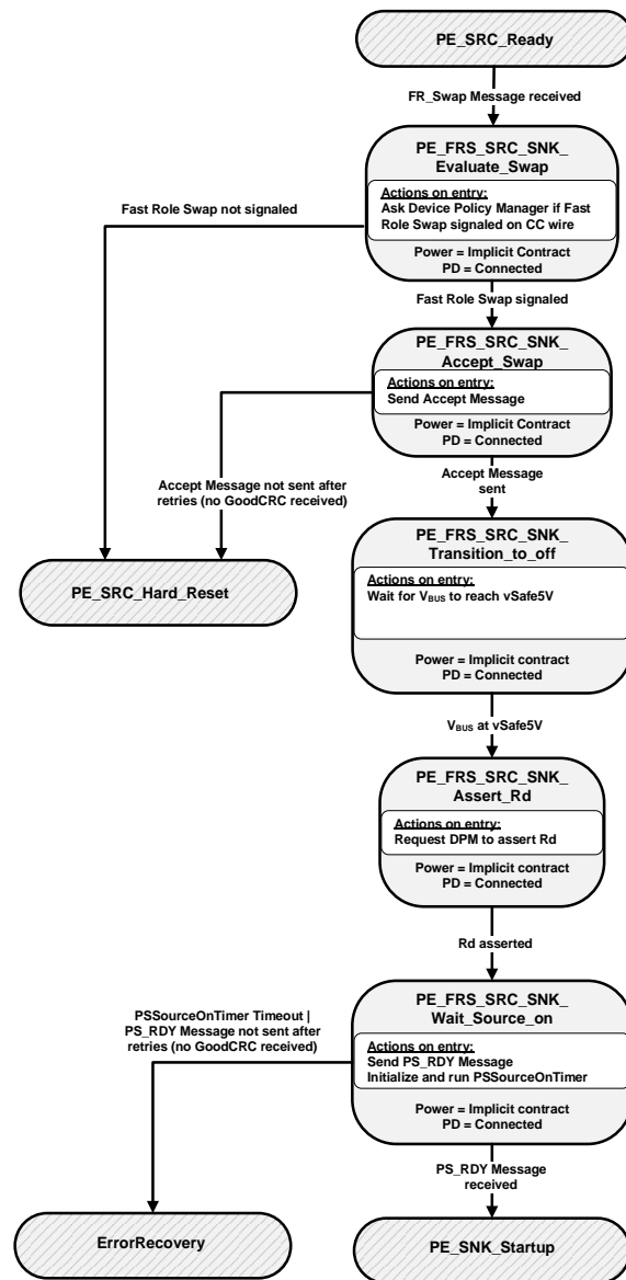
Figure 8-151: Dual-Role Port in Source to Sink Fast Role Swap State Diagram
