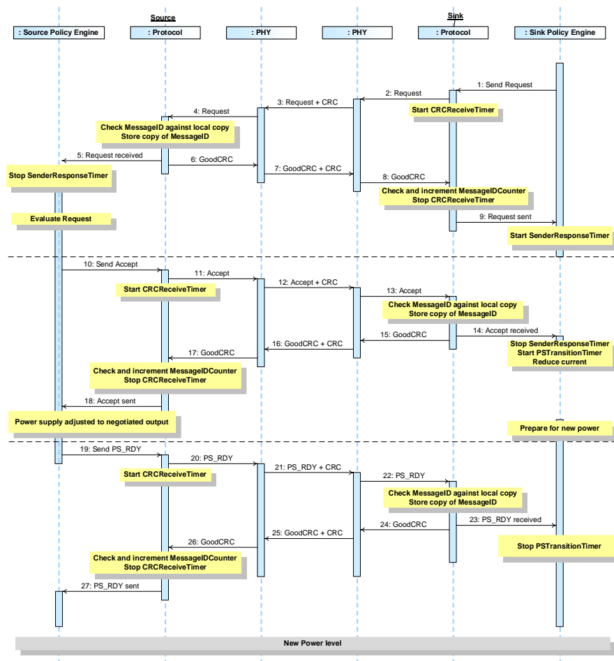
Figure 8-8 SPR Sink Makes Request (Accept)
