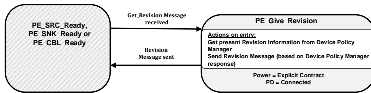
Figure 8-138 Give Revision State Diagram
