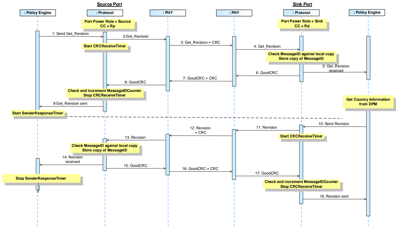
Figure 8-71 Source Gets Sink's Revision Information
