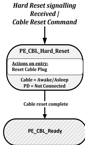
Figure 8-176 Cable Plug Hard Reset State Diagram
