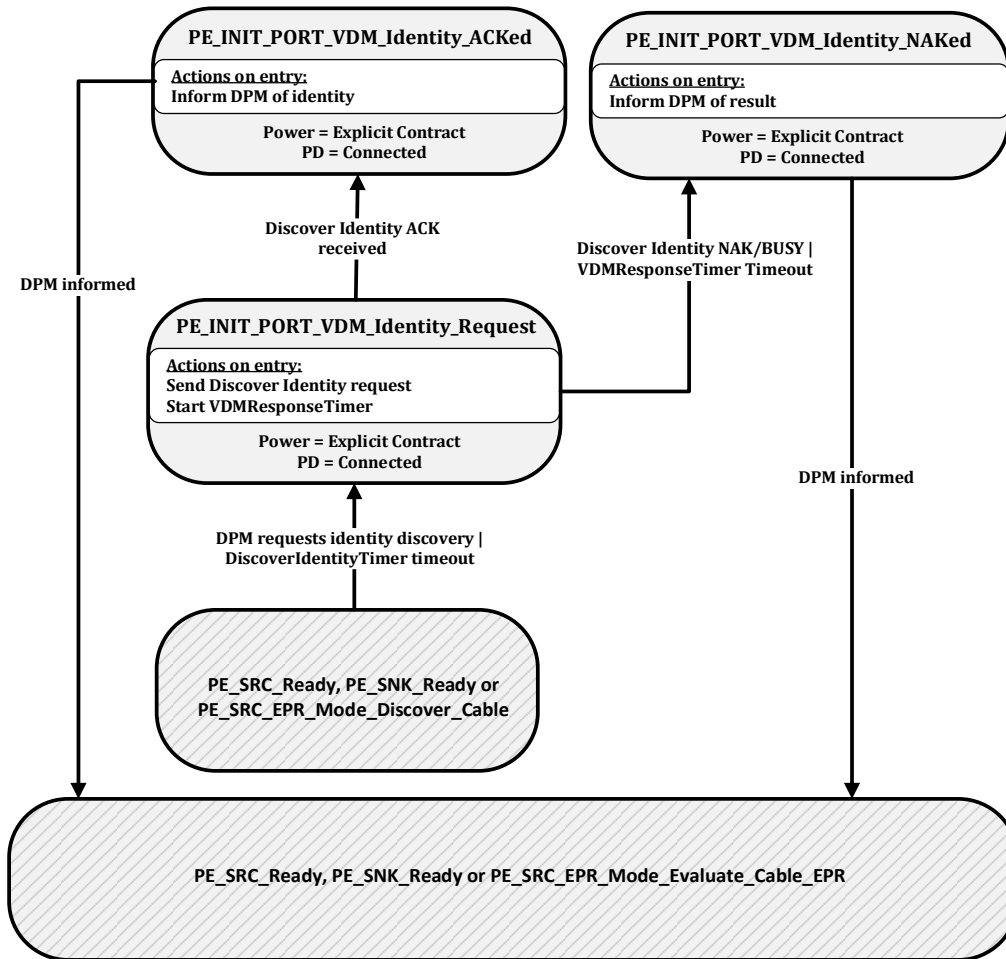
Figure 8-162 Initiator to Port VDM Discover Identity State Diagram
