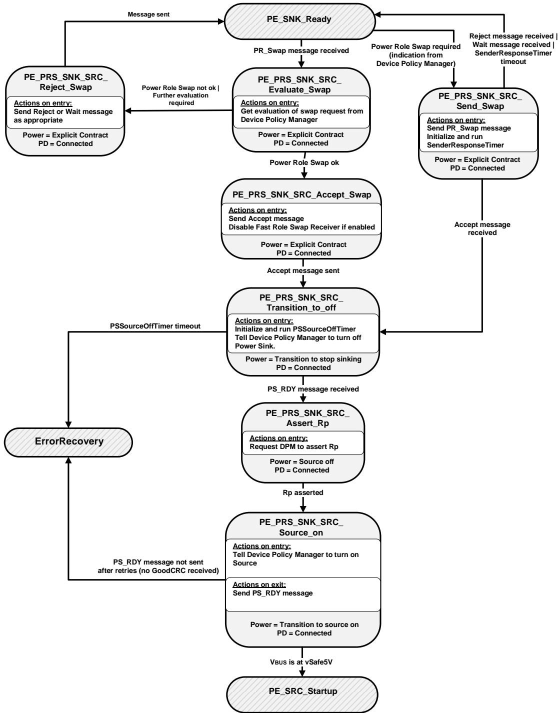
Figure 8-150: Dual-role Port in Sink to Source Power Role Swap State Diagram
