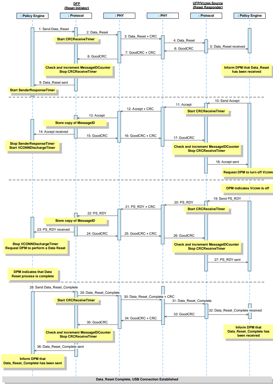
Figure 8-24 DFP Initiated Data Reset where the UFP is the Vconn Source
