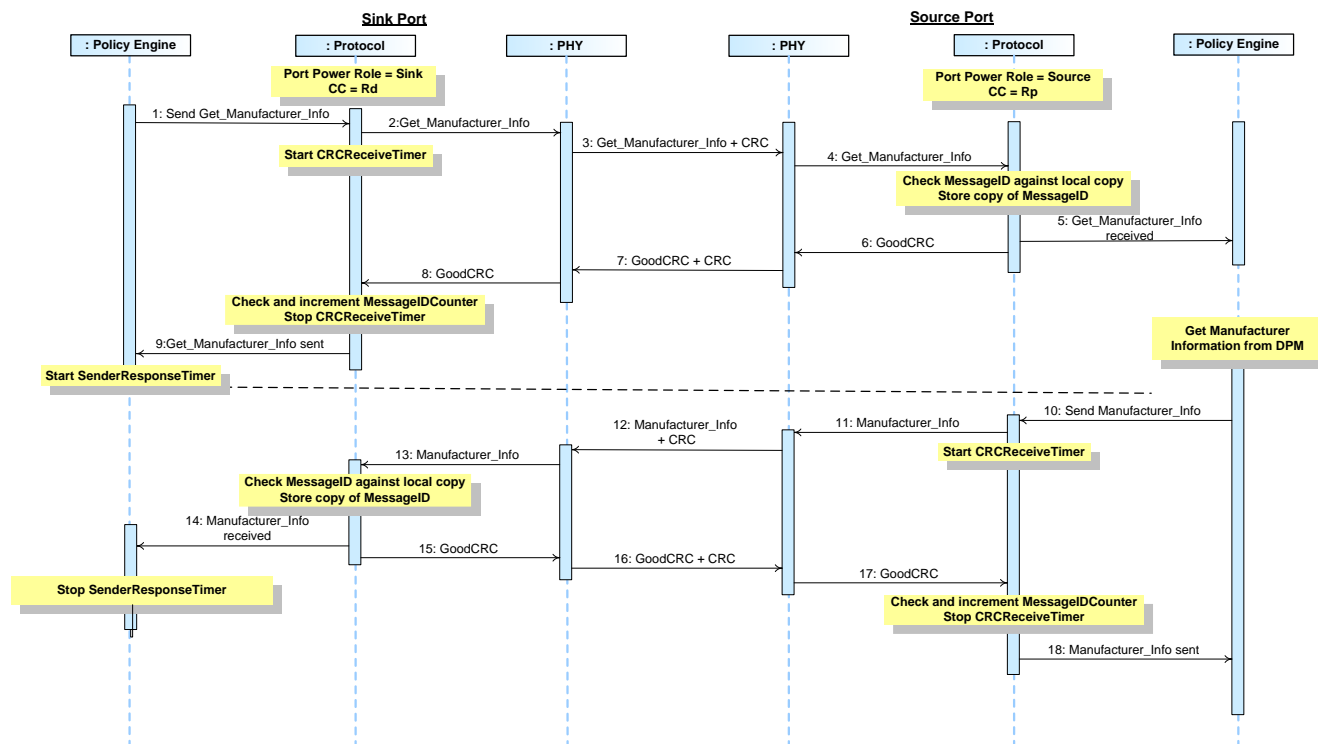
Figure 8-61 Sink Gets Source's Port Manufacturer Information
