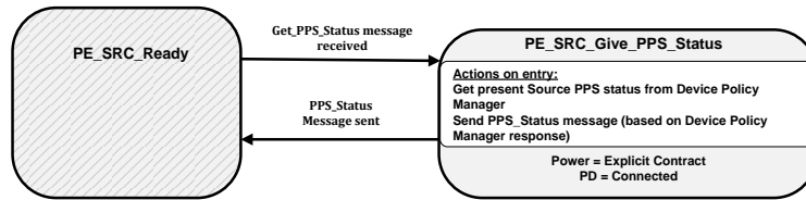
Figure 8-126 Source Give Source PPS Status State Diagram
