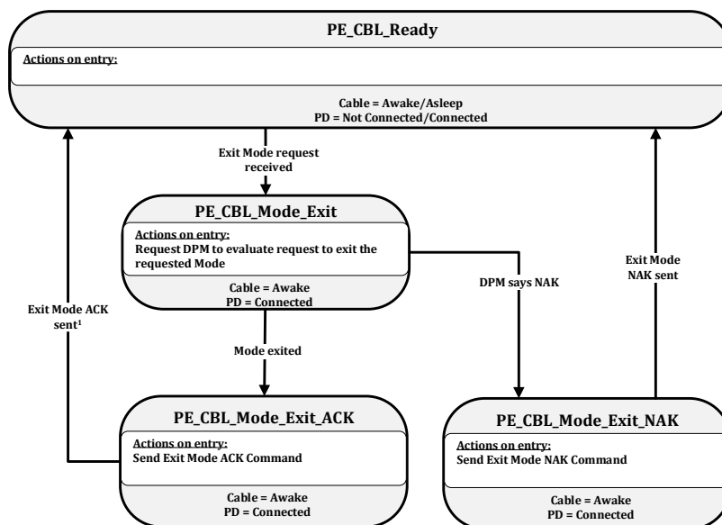
Figure 8-181 Cable Plug Structured VDM Exit Mode State Diagram
