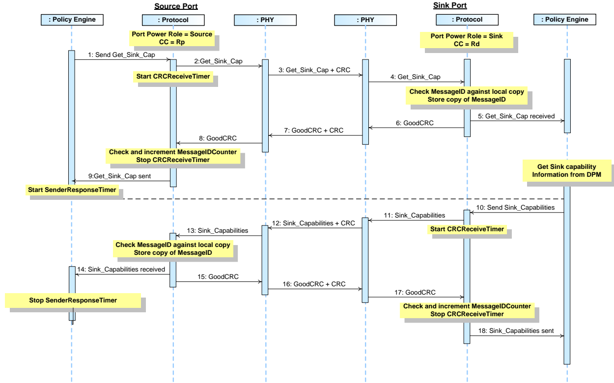
Figure 8-46 Source Gets Sink's Capabilities
