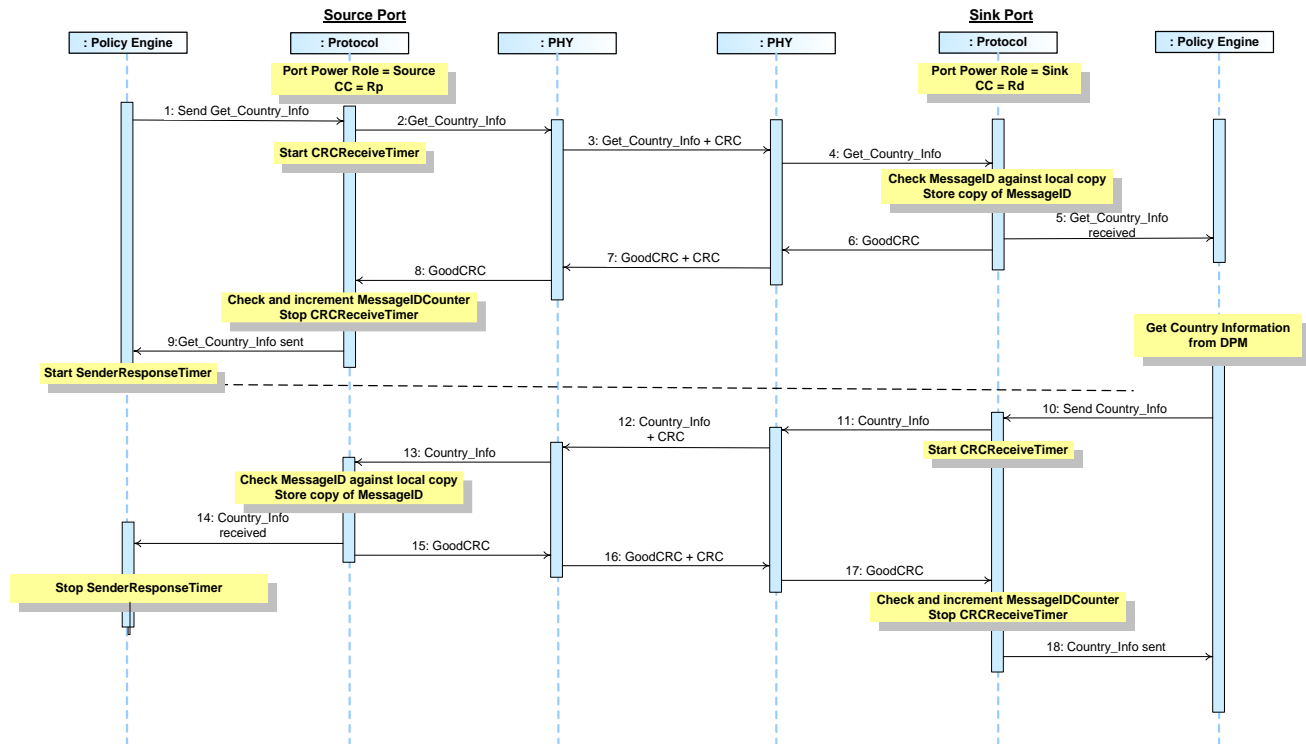
Figure 8-68 Source Gets Sink's Country Information
