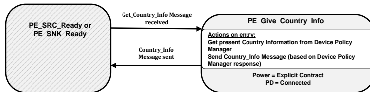
Figure 8-136 Give Country Information State Diagram
