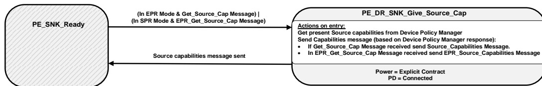
Figure 8-156 Dual-Role (Sink) Give Source Capabilities State Diagram
