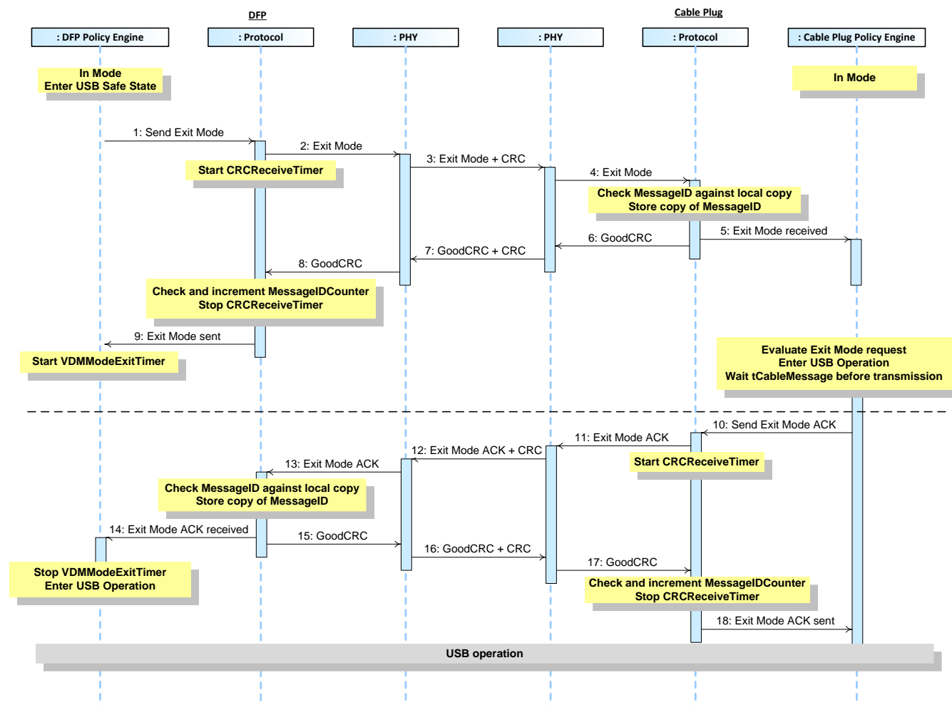
Figure 8-90 DFP to Cable Plug Exit Mode
