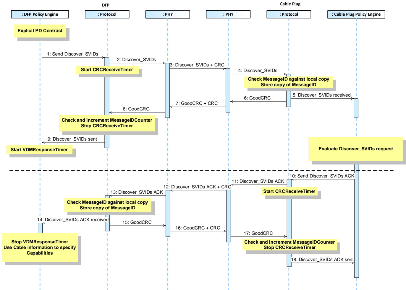
Figure 8-84 DFP to Cable Plug Discover SVIDs
