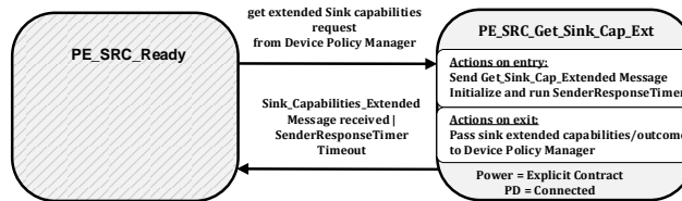
Figure 8-121 Source Port Get Sink Capabilities Extended State Diagram
