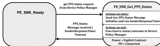
Figure 8-125 Sink Port Get Source PPS Status State Diagram
