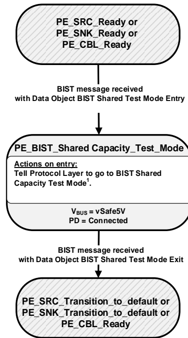
Figure 8-188 BIST Shared Capacity Test Mode State Diagram
