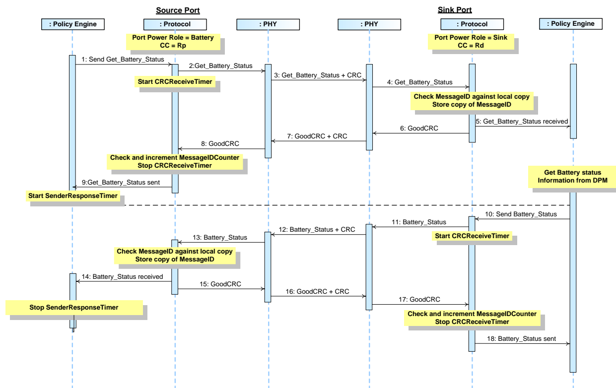
Figure 8-59 Source Gets Sink's Battery Status
