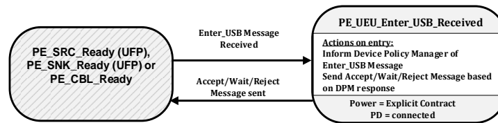
Figure 8-140 UFP Enter_USB Message State Diagram
