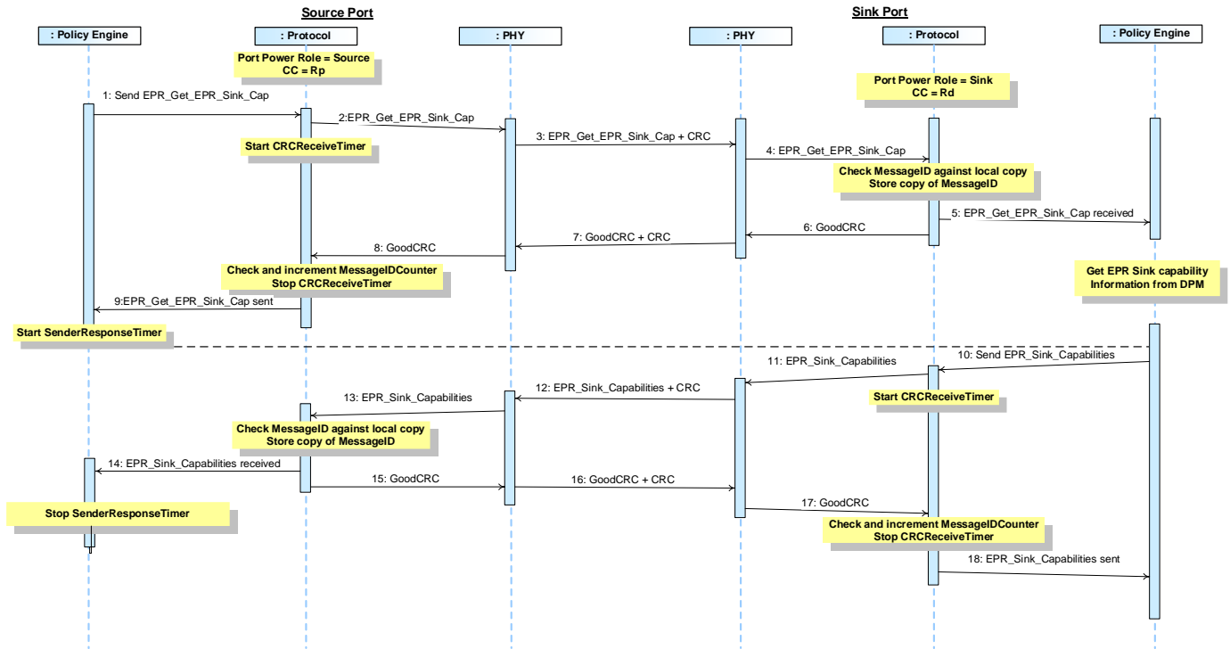
Figure 8-50 Source Gets Sink's EPR Capabilities
