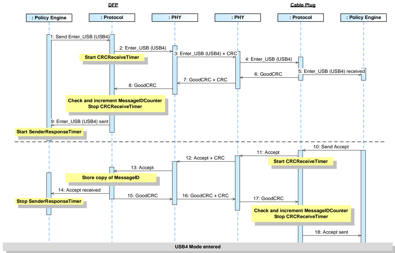
Figure 8-96 Cable Plug Entering USB4 Mode (Valid)
