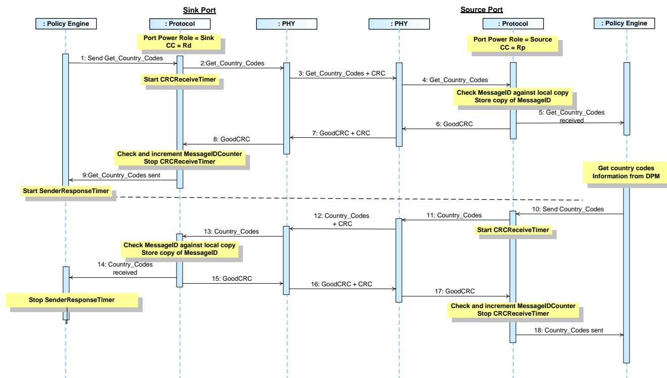
Figure 8-66 Sink Gets Source's Country Codes
