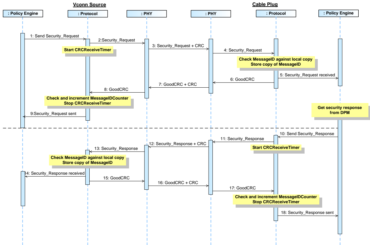
Figure 8-76 VCONN Source requests security exchange with Cable Plug
