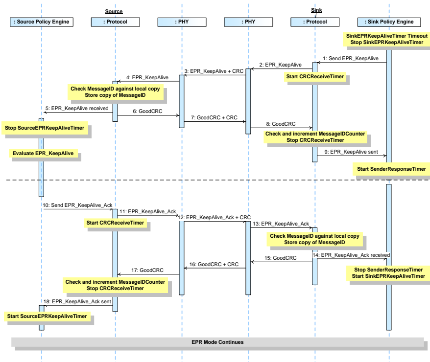
Figure 8-15 EPR Keep Alive
