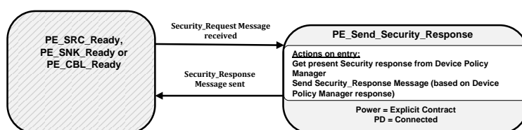
Figure 8-142 Send security response State Diagram
