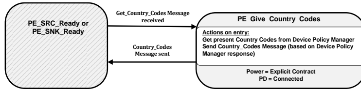
Figure 8-134 Give Country Codes State Diagram
