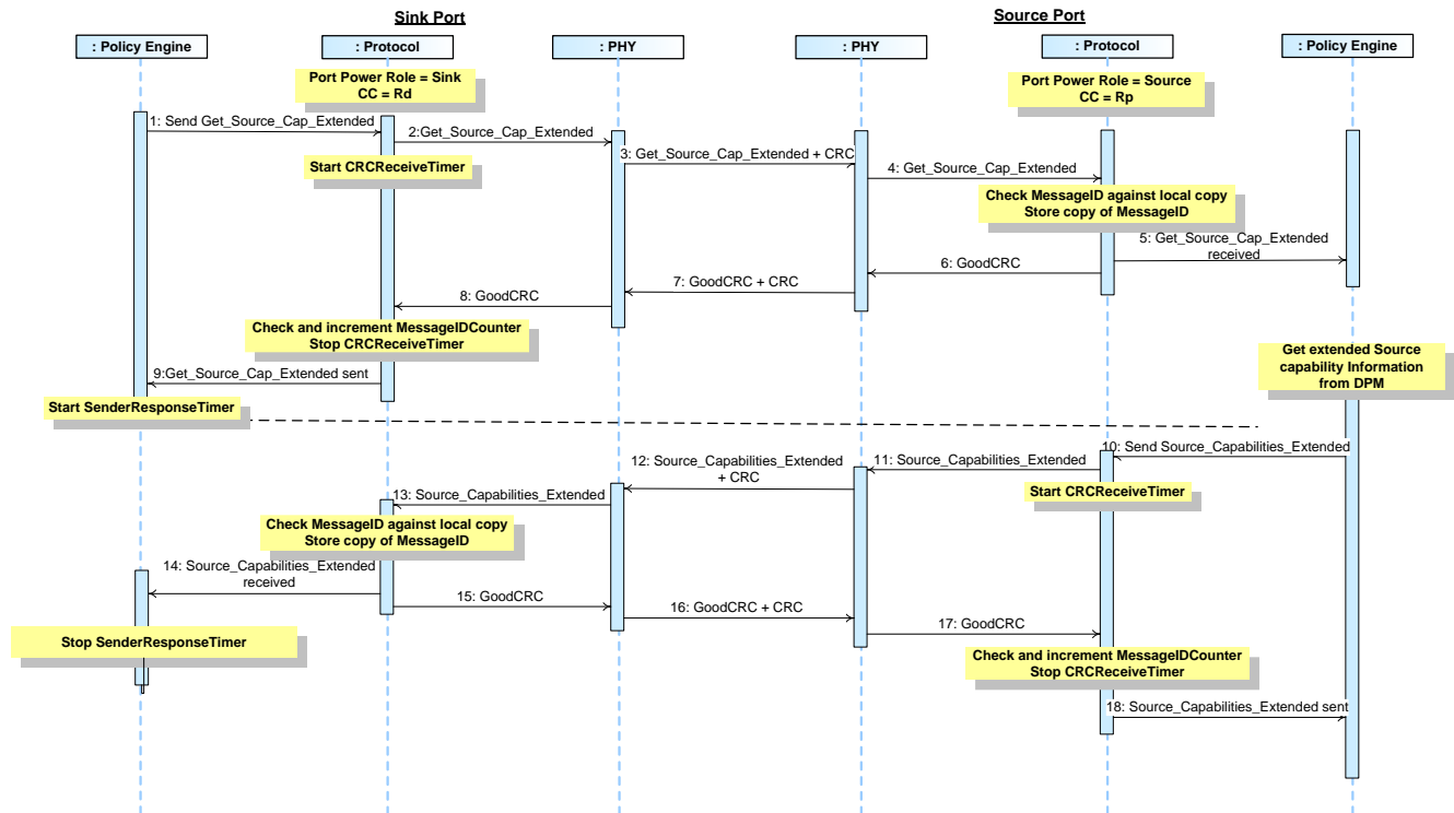
Figure 8-52 Sink Gets Source's Extended Capabilities
