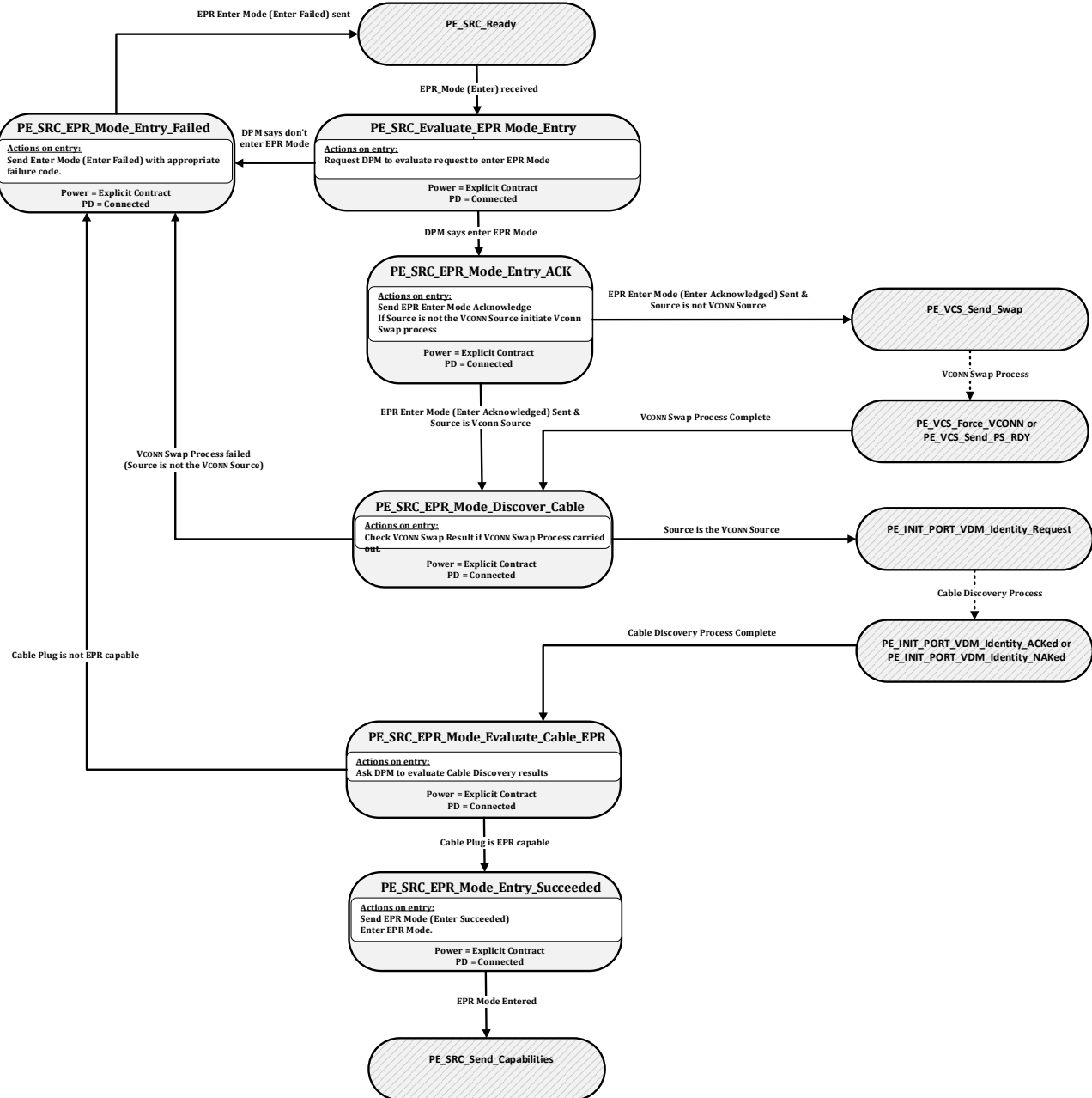
Figure 8-182 Source EPR Mode Entry State Diagram
