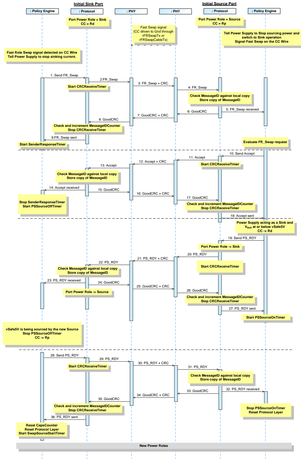
Figure 8-31 Successful Fast Role Swap Sequence
