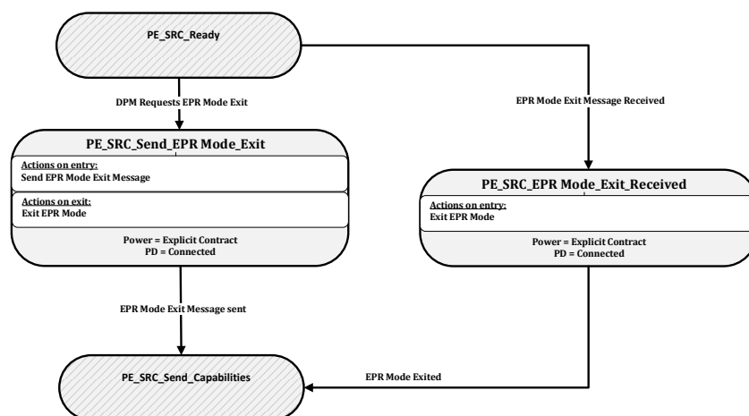
Figure 8-184 Source EPR Mode Exit State Diagram
