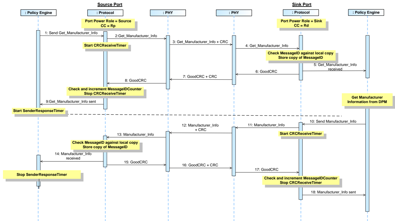
Figure 8-60 Source Gets Sink's Port Manufacturer Information
