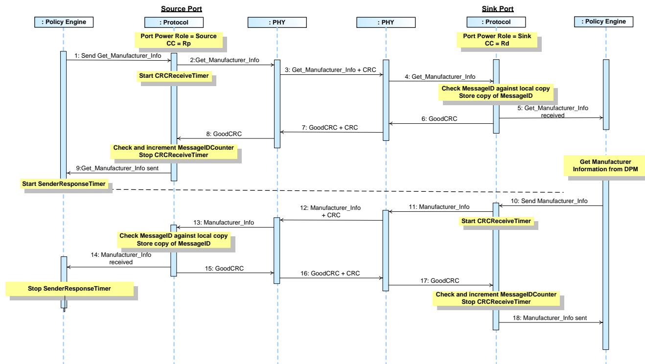
Figure 8-62 Source Gets Sink's Battery Manufacturer Information
