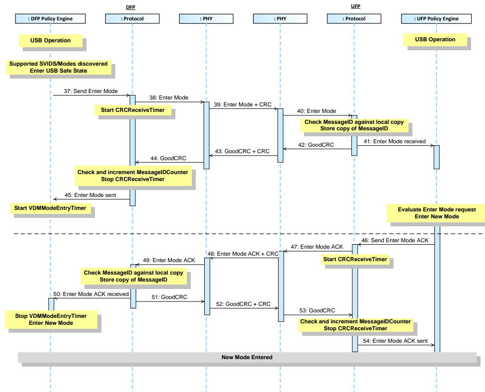
Figure 8-87 DFP to UFP Enter Mode
