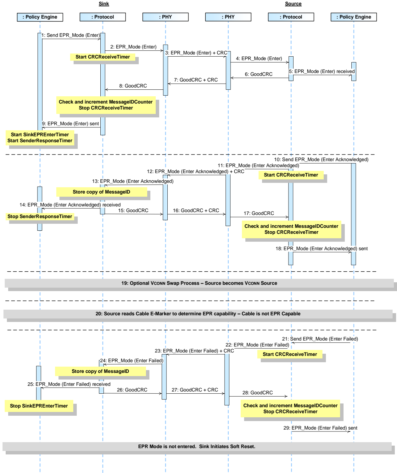
Figure 8-12 Entering EPR Mode (Failure due to non-EPR cable)
