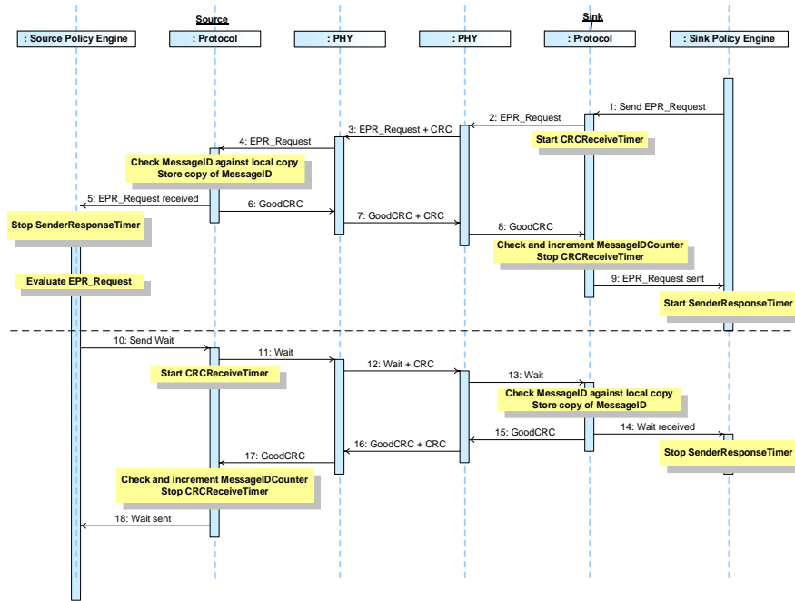
Figure 8-20 EPR Sink Makes Request (Wait)
