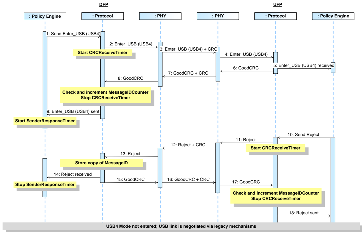
Figure 8-97 UFP Entering USB4 Mode (Invalid)
