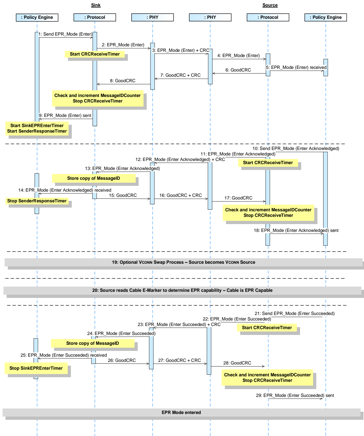
Figure 8-11 Entering EPR Mode (Success)
