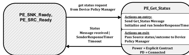
Figure 8-123 Get Status State Diagram
