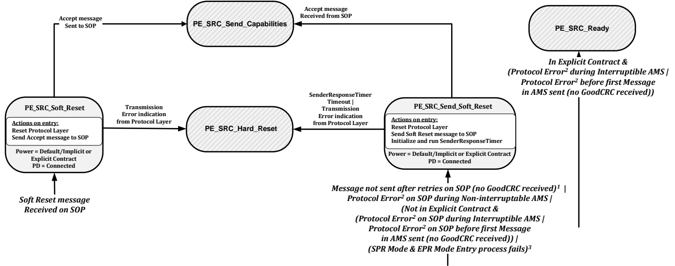
Figure 8-108 SOP Source Port Soft Reset and Protocol Error State Diagram
