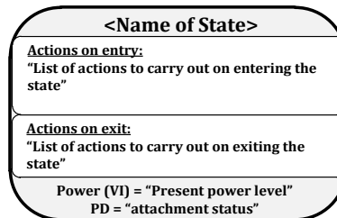
Figure 8-101 Outline of States
