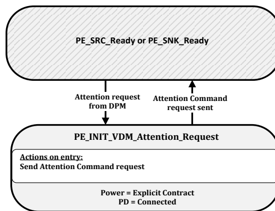
Figure 8-165 Initiator VDM Attention State Diagram
