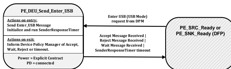
Figure 8-139 DFP Enter_USB Message State Diagram
