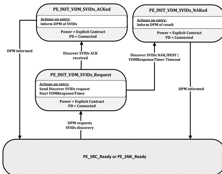
Figure 8-163 Initiator VDM Discover SVIDs State Diagram
