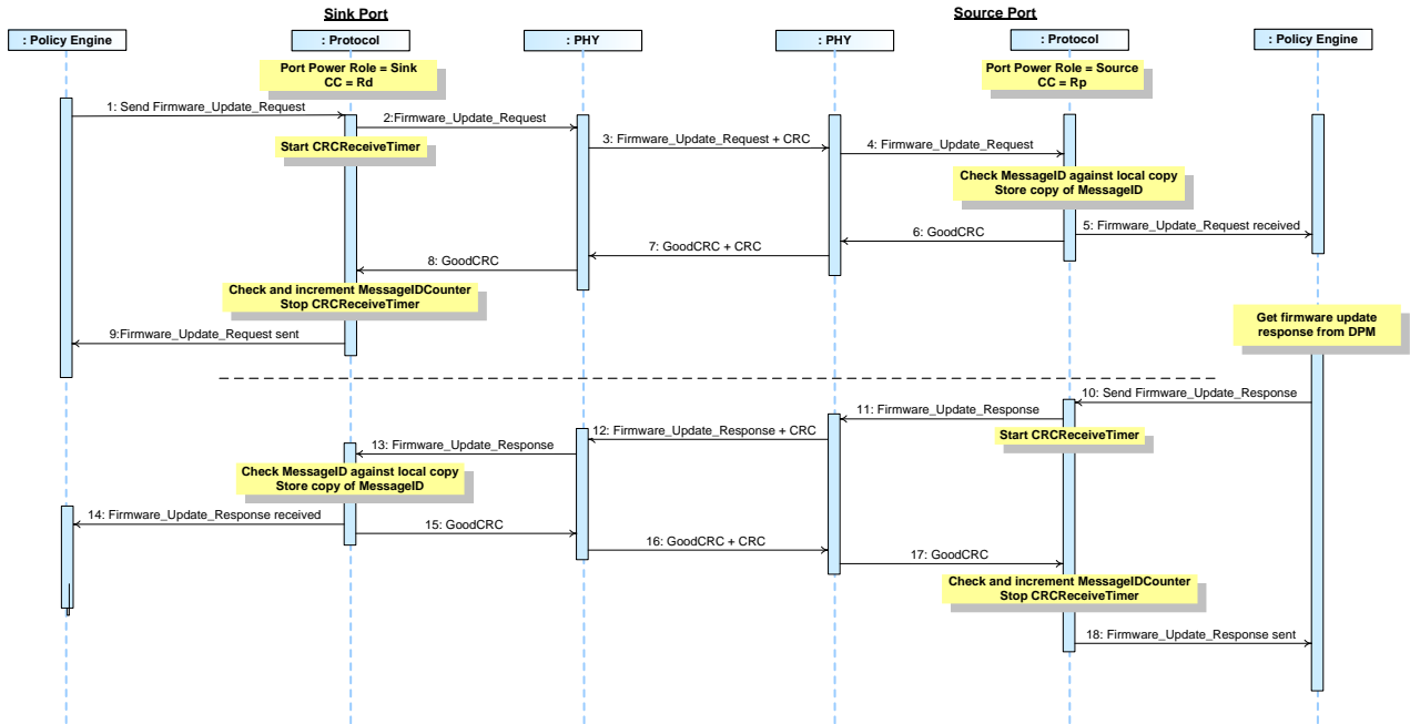
Figure 8-78 Sink requests firmware update exchange with Source
