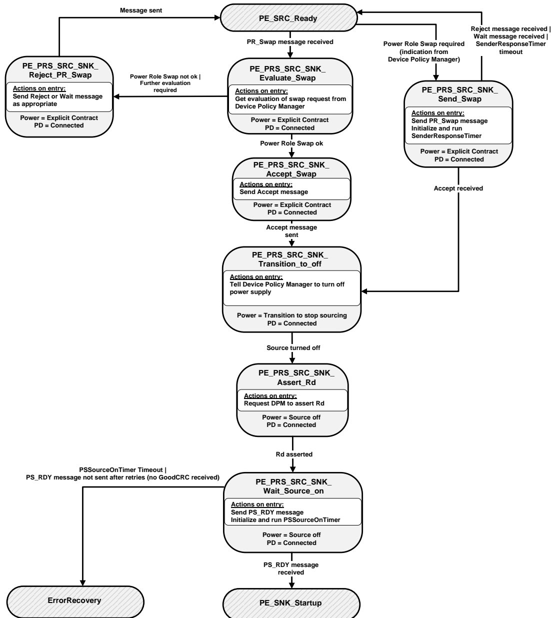
Figure 8-149: Dual-Role Port in Source to Sink Power Role Swap State Diagram
