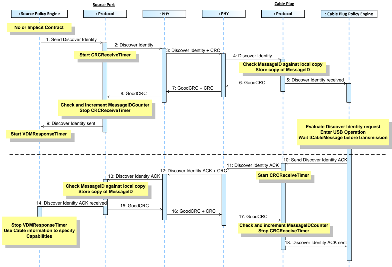
Figure 8-81 Source Port to Cable Plug Discover Identity
