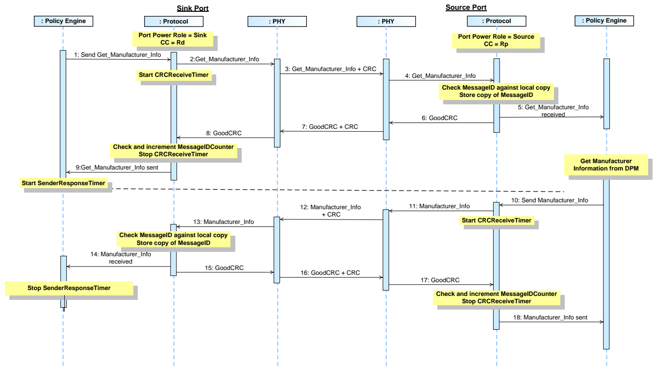
Figure 8-63 Sink Gets Source's Battery Manufacturer Information
