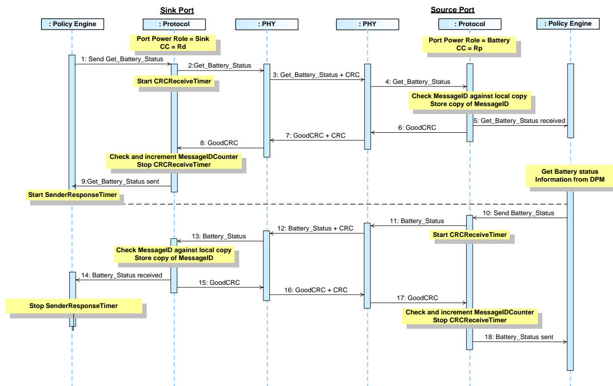
Figure 8-58 Sink Gets Source's Battery Status
