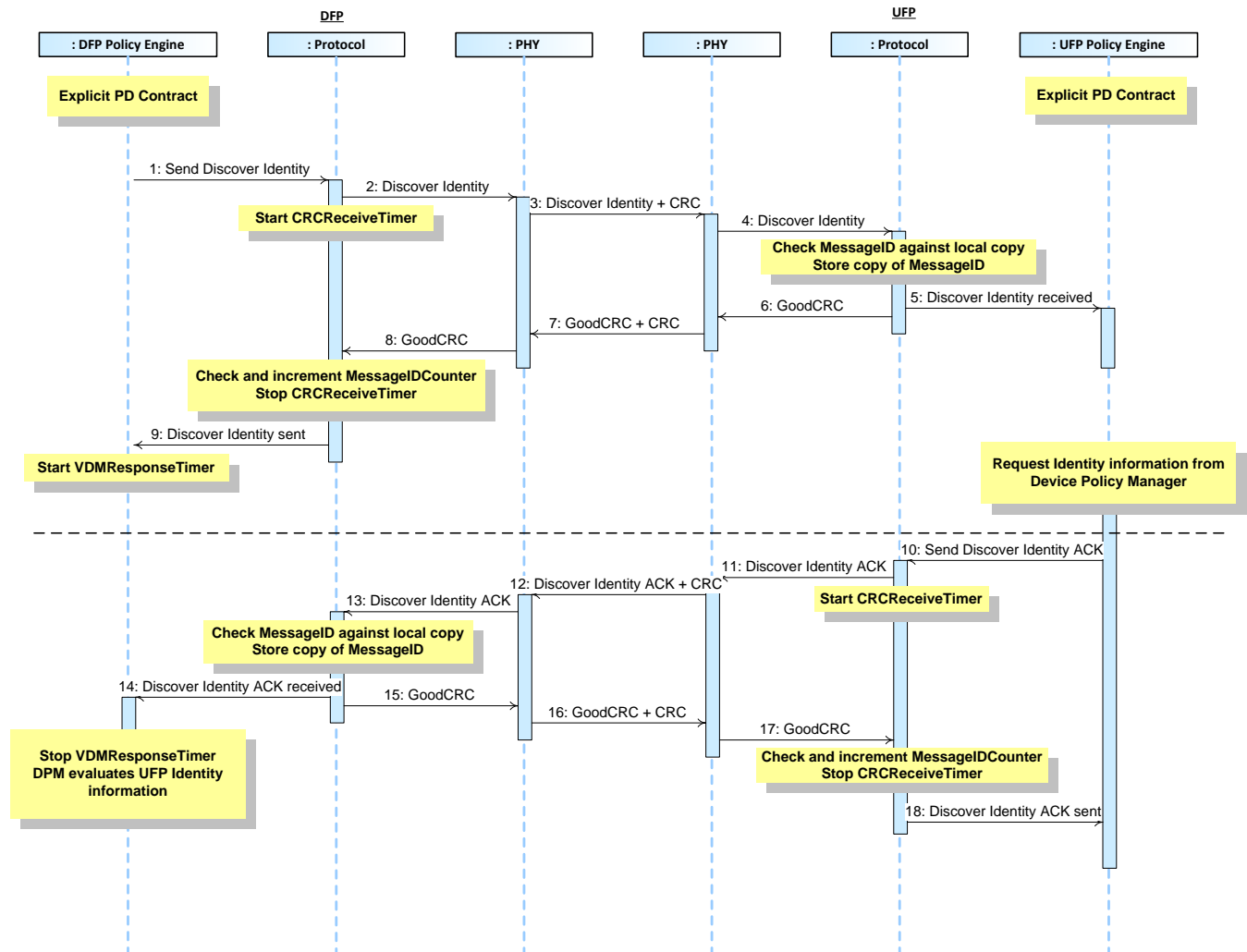
Figure 8-80 DFP to UFP Discover Identity
