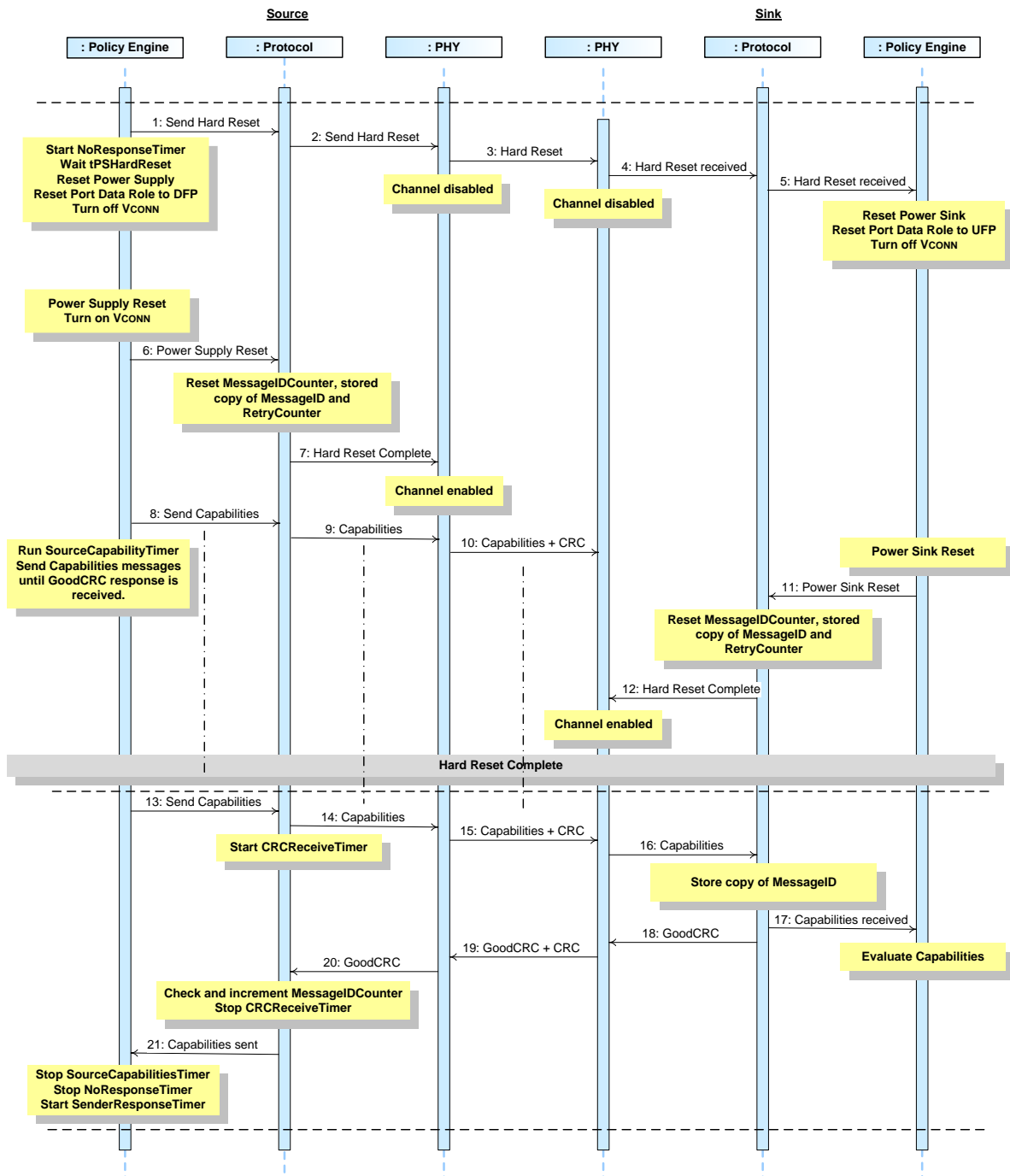
Figure 8-28 Source initiated reset - Sink long reset
