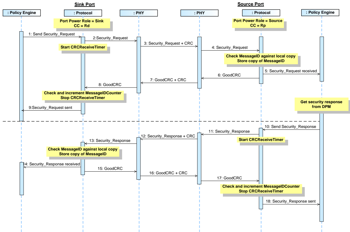
Figure 8-75 Sink requests security exchange with Source
