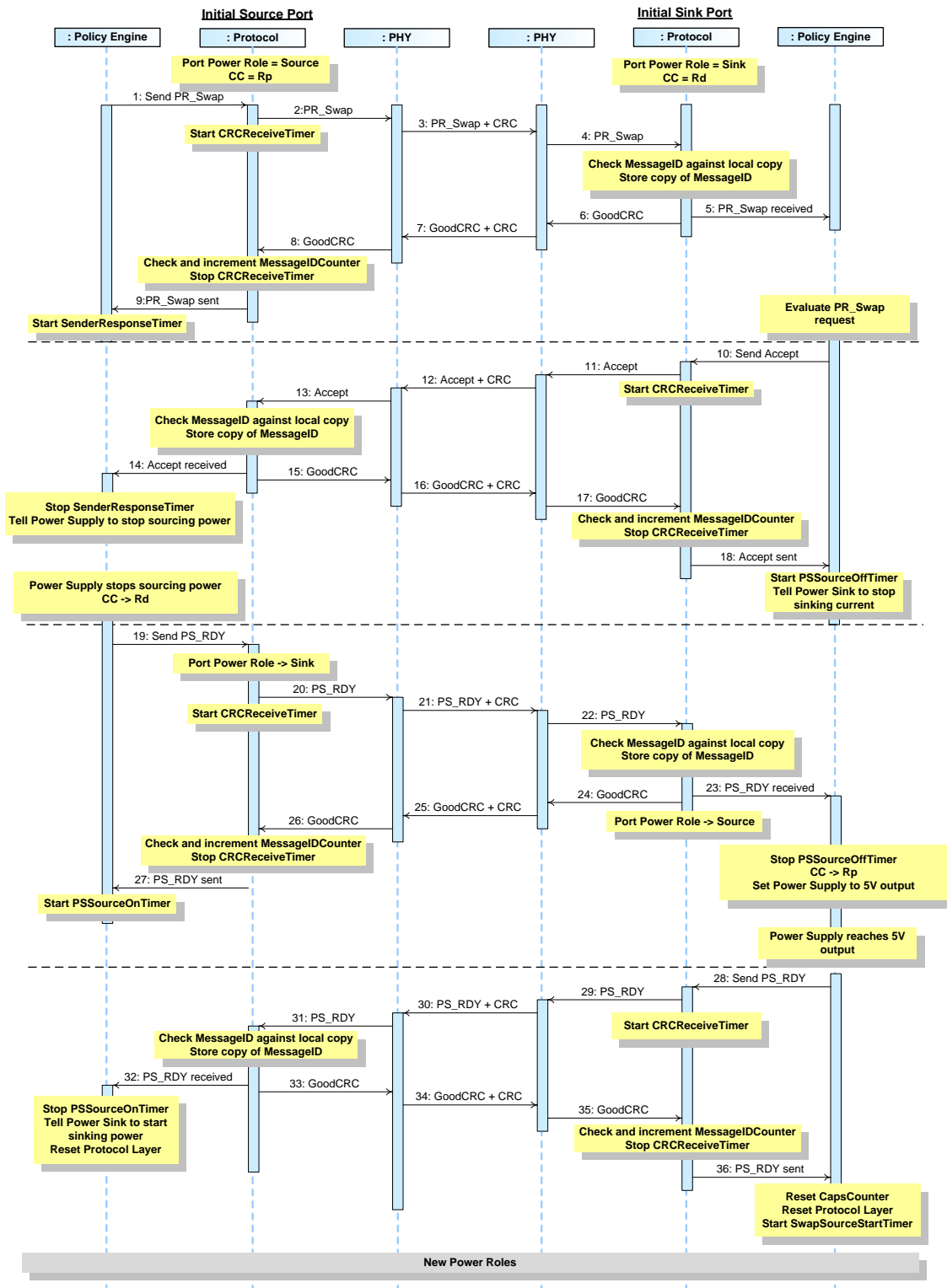
Figure 8-29 Successful Power Role Swap Sequence Initiated by the Source
