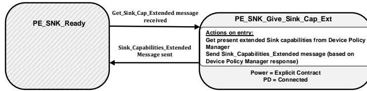
Figure 8-122 Sink Give Sink Capabilities Extended State Diagram
