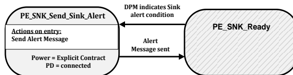
Figure 8-117 Sink Port Sink Alert State Diagram
