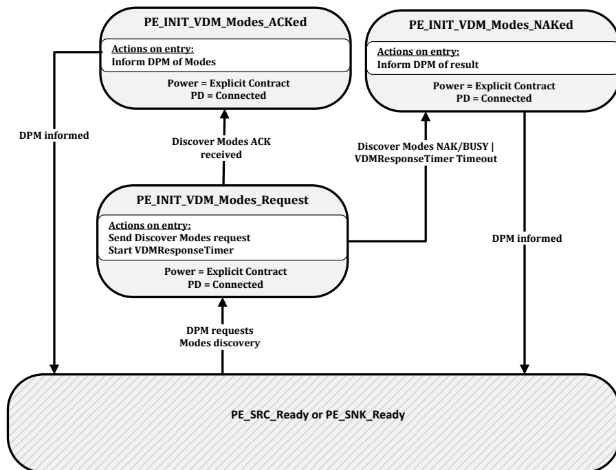
Figure 8-164 Initiator VDM Discover Modes State Diagram
