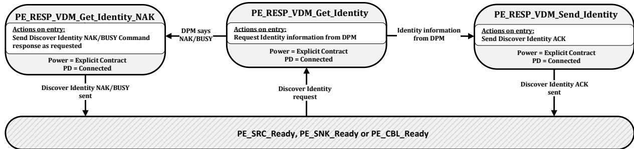
Figure 8-166 Responder Structured VDM Discover Identity State Diagram
