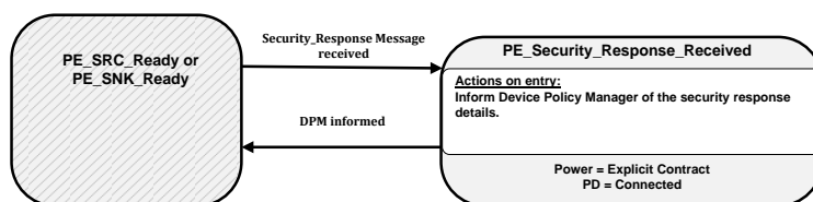
Figure 8-143 Security response received State Diagram
