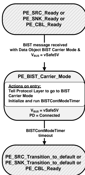
Figure 8-186 BIST Carrier Mode State Diagram
