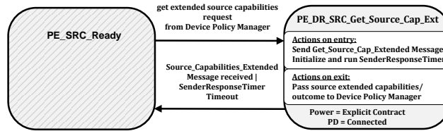
Figure 8-157 Dual-Role (Source) Get Source Capabilities Extended State Diagram
