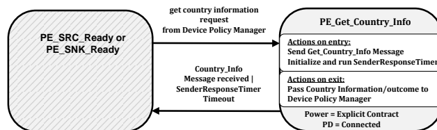
Figure 8-135 Get Country Information State Diagram
