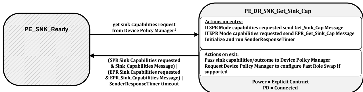
Figure 8-155 Dual-Role (Sink) Get Sink Capabilities State Diagram
