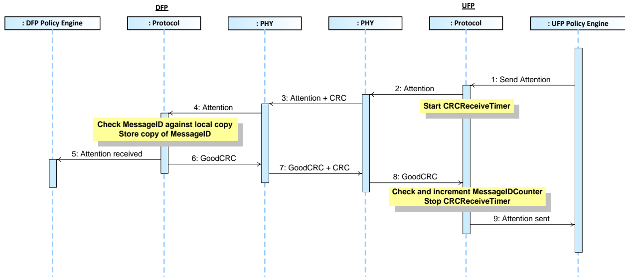
Figure 8-91 UFP to DFP Attention
