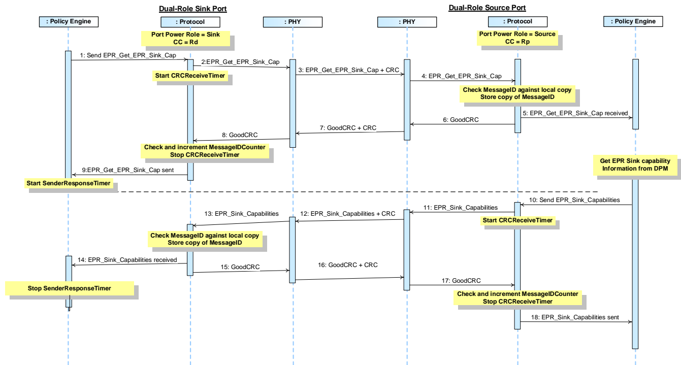
Figure 8-51 Dual-Role Sink Gets Dual-Role Source's Capabilities as an EPR Sink
