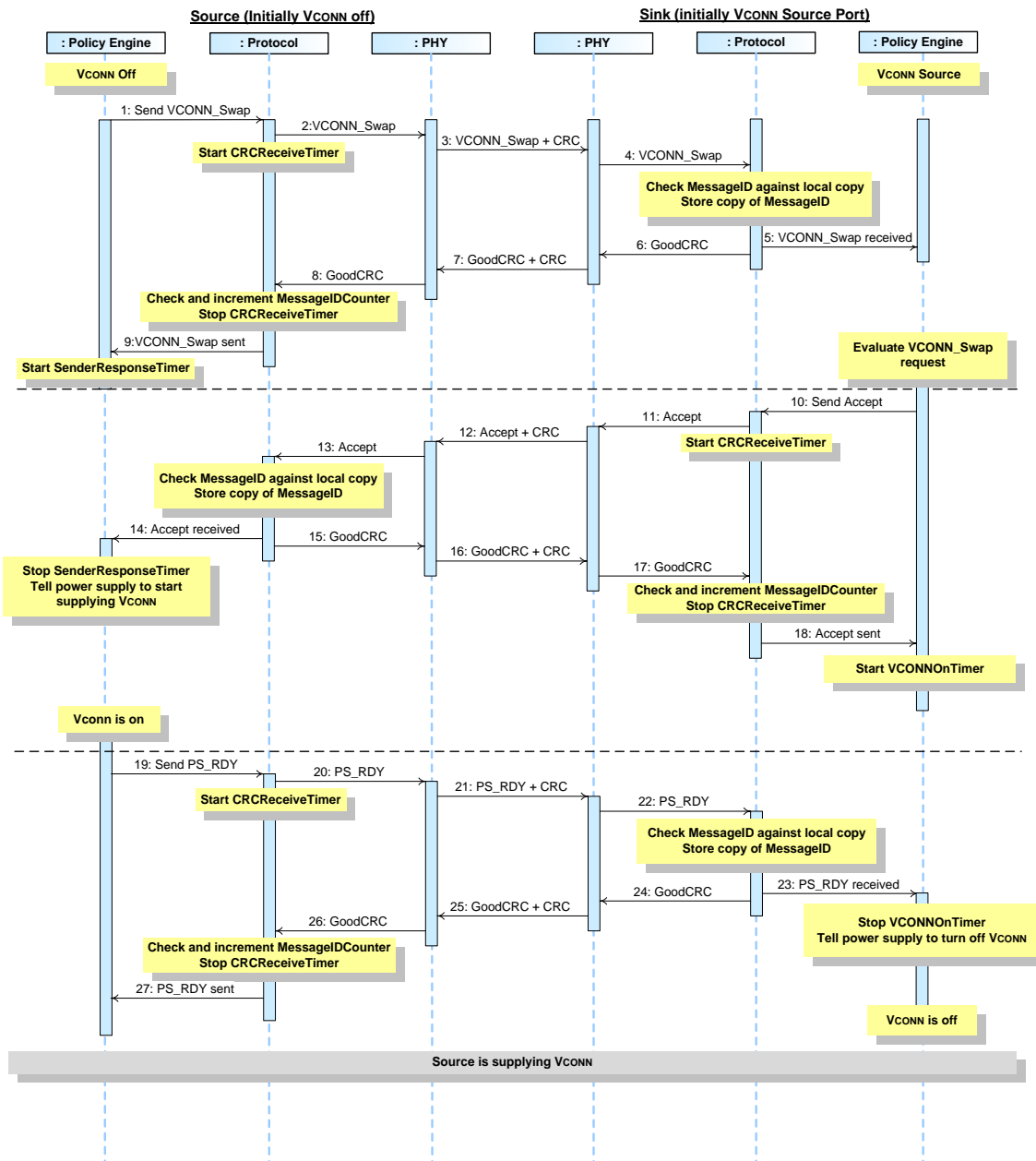
Figure 8-37 Sink to Source VCONN Source Swap
