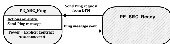
Figure 8-114 Source Port Ping State Diagram
