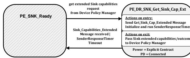
Figure 8-159 Dual-Role (Sink) Get Sink Capabilities Extended State Diagram
