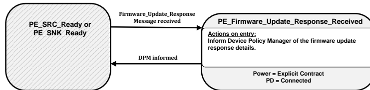
Figure 8-146 Firmware update response received State Diagram
