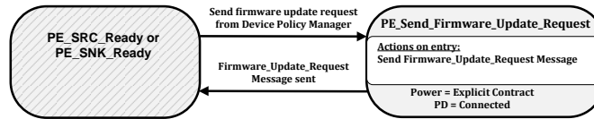
Figure 8-144 Send firmware update request State Diagram
