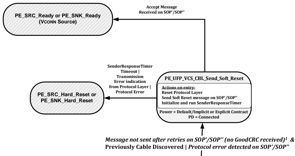
Figure 8-178 UFP/VCONN Source Soft Reset of a Cable Plug or VPD State Diagram
