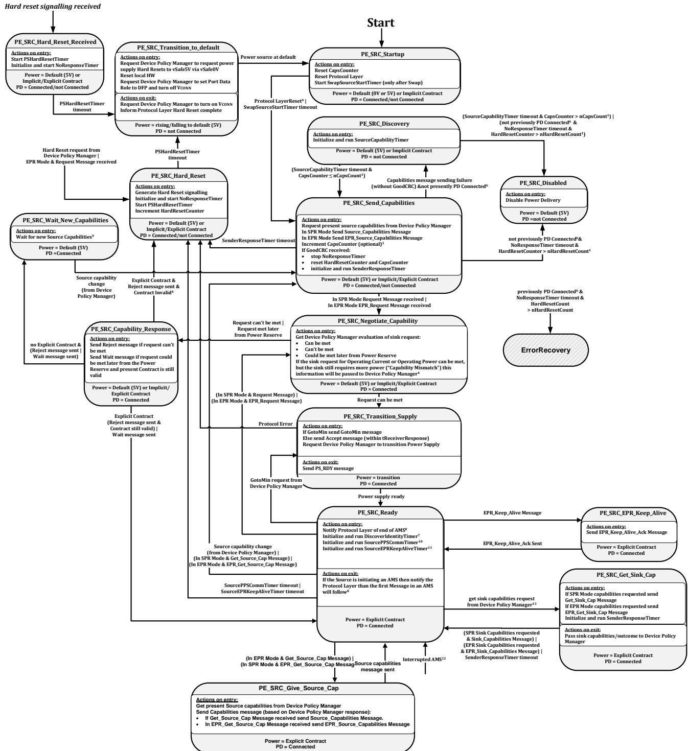
Figure 8-106 Source Port Policy Engine State Diagram
