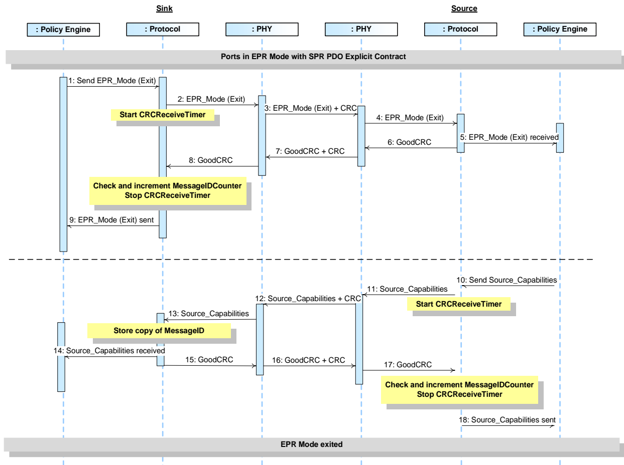
Figure 8-16 Exiting EPR Mode (Sink Initiated)
