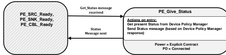
Figure 8-124 Source Give Source Status State Diagram
