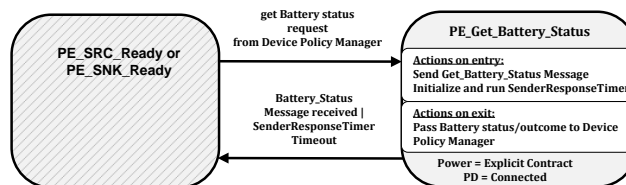
Figure 8-129 Get Battery Status State Diagram
