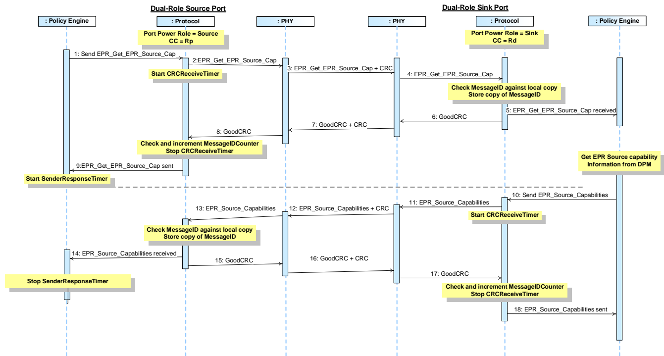
Figure 8-49 Dual-Role Source Gets Dual-Role Sink's Capabilities as an EPR Source
