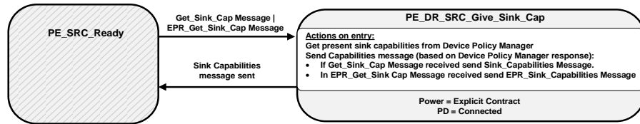
Figure 8-154 Dual-Role (Source) Give Sink Capabilities diagram
