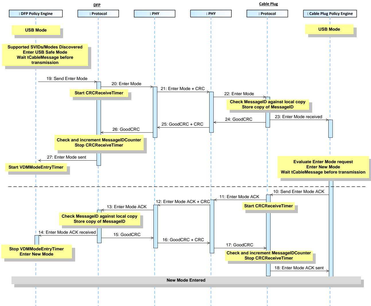
Figure 8-89 DFP to Cable Plug Enter Mode
