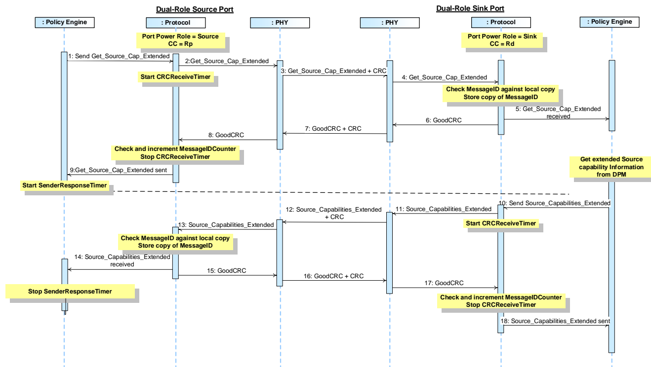
Figure 8-53 Dual-Role Source Gets Dual-Role Sink's Extended Capabilities
