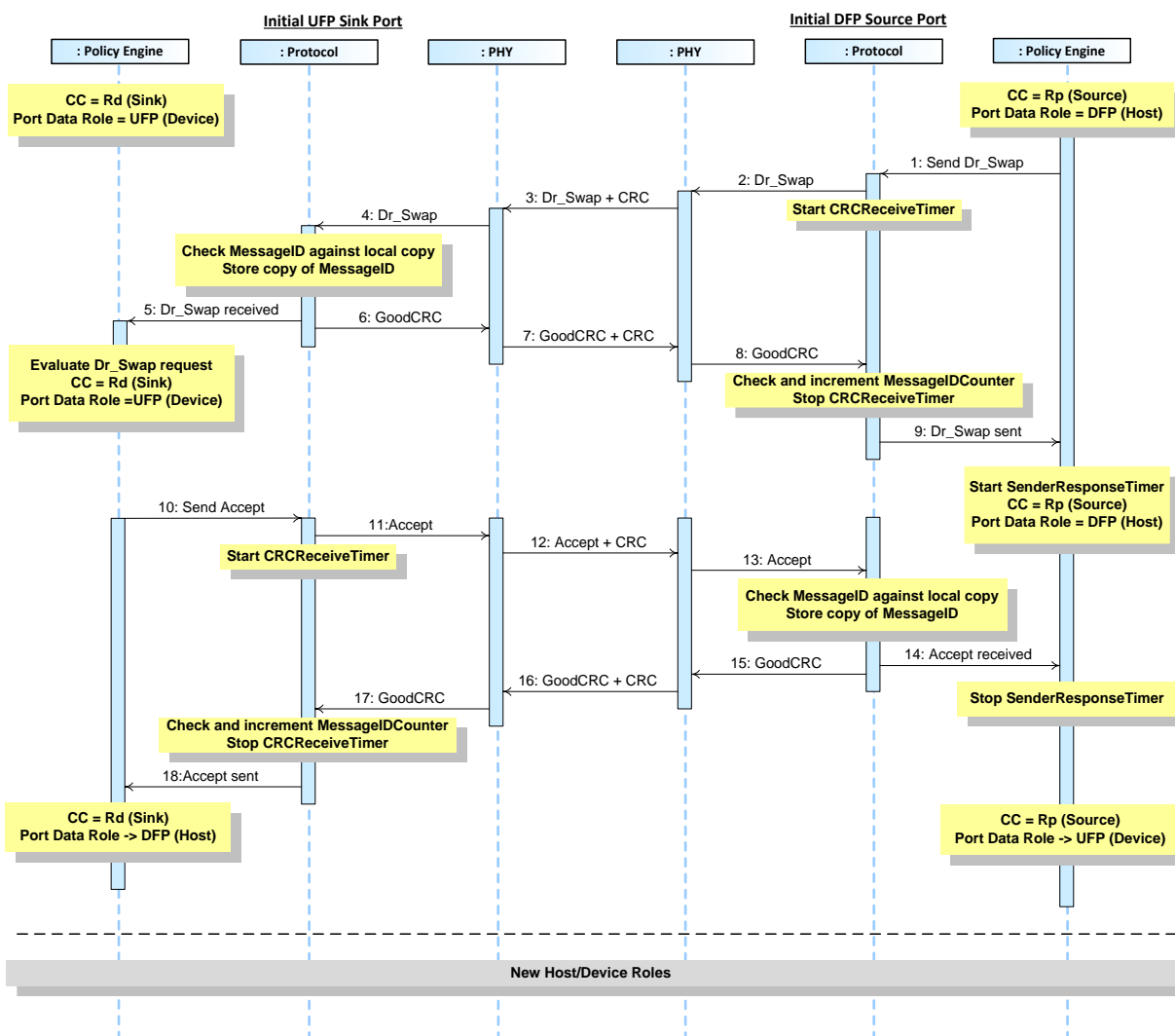
Figure 8-34 Data Role Swap, DFP operating as Source initiates
