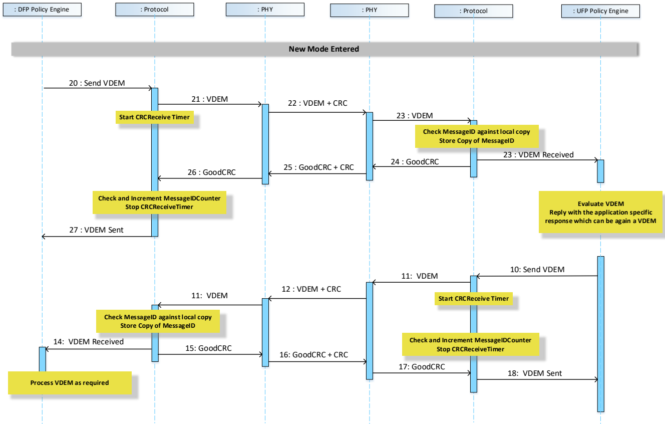
Figure 8-100 Unstructured VDEM Message Sequence
