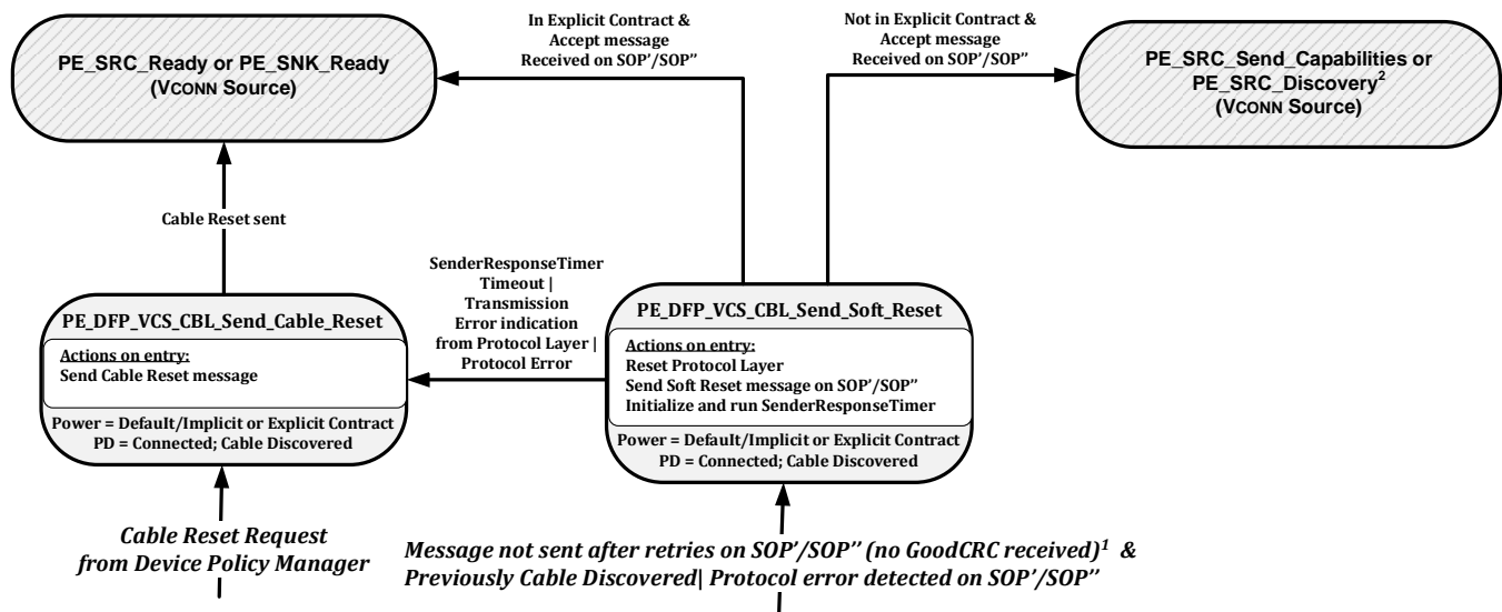
Figure 8-177 DFP/VCONN Source Soft Reset or Cable Reset of a Cable Plug or VPD State Diagram
