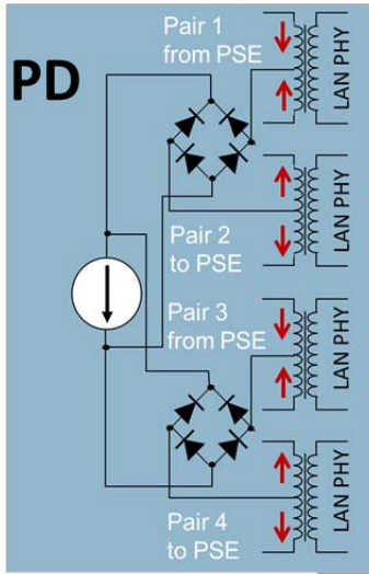
Figure 2.2 PD Connection
