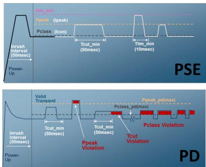
Figure 2.11 Power Regulation and PD Overloads
