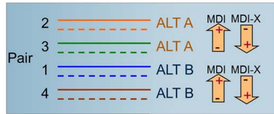
Figure 2.3 PSE Pairsets
