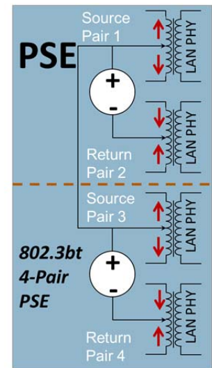
Figure 2.1 PSE Connection
