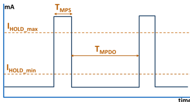
Figure 2.13 DC MPS Minimum Power State
