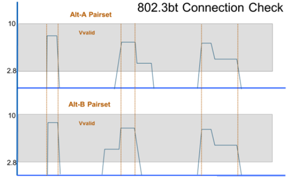
Figure 2.5 802.3bt Connection Check
