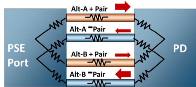
Figure 2.11 Pair-to-Pair Current Unbalance
