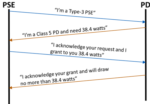
Figure 2.10 PoE LLDP Dialog/Negotiation
