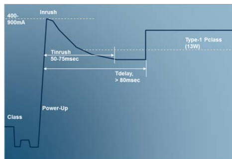
Figure 2.9 PD Inrush and Power Delay
