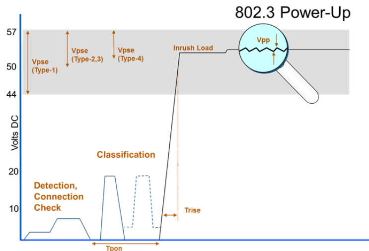
Figure 2.8 802.3 Power-Up
