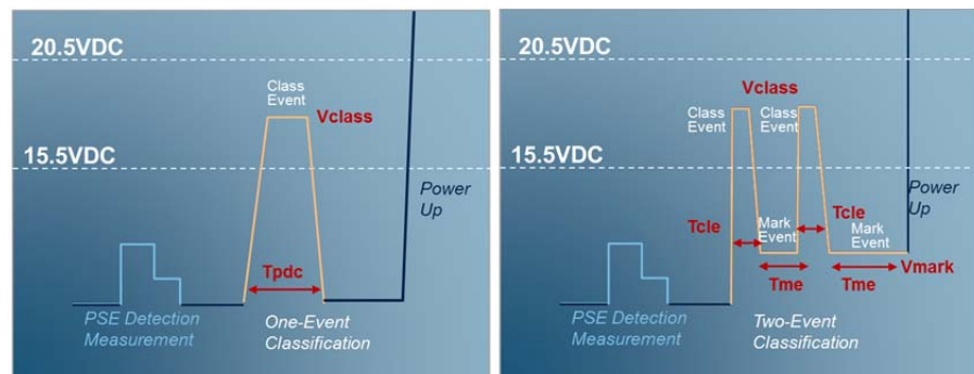
Figure 2.6 PD Classification under the 802.3at Specification
