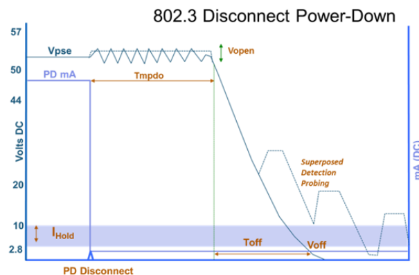
Figure 2.12 802.3 PoE Disconnect Power-Down
