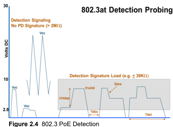
Figure 2.4 802.3 PoE Detection
