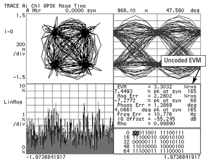
Figure 7. Uncoded EVM measurement on a cdma2000 SR1 pilot signal (forward link)
