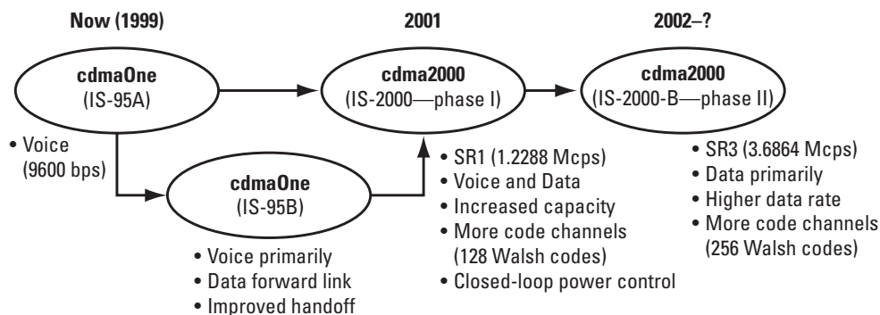
Figure 1. Evolution from cdmaOne to cdma2000
