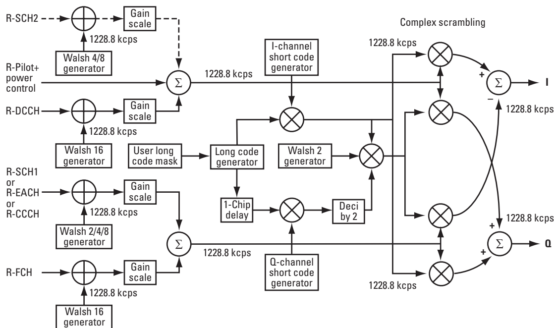
Figure 16. Channel summing and HPSK spreading in cdma2000 reverse link (SR1)
