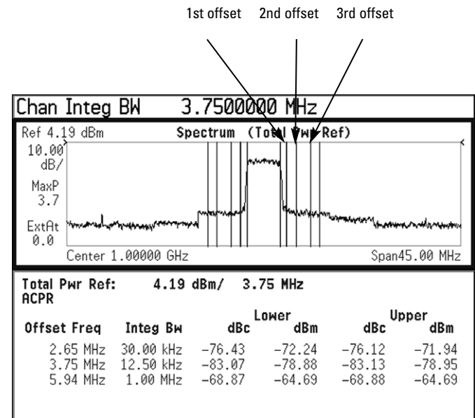
Figure 5. ACPR measurement for a cdma2000 SR3 DS signal
