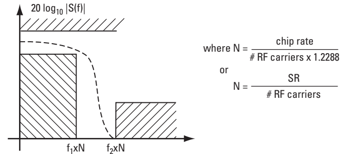
Figure 4. Proposed limits for cdma2000 baseband filters
