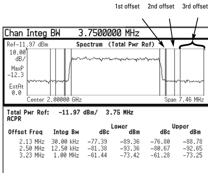
Figure 3. ACPR measurement for a cdma2000 SR3 MC signal
