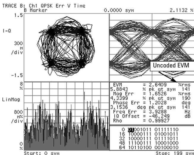
Figure 13. EVM (uncoded) on a cdma2000 SR1 reverse link signal with R-Pilot and R-FCH (RC3 at 9.6 kbps) activated. Both channels are at the same power level
