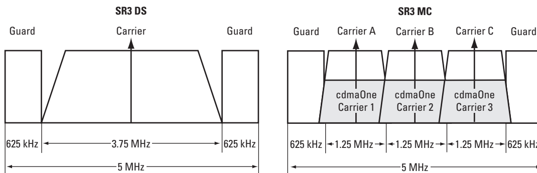
Figure 2. Bandwidth limits for SR3DS and SR3 MC
