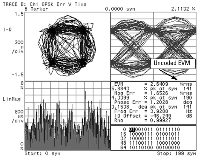
Figure 14. EVM (uncoded) on a cdma2000 SR1 reverse link signal with R-Pilot and R-FCH (RC3 at 9.6 kbps) activated. The power level for R-FCH is 7.5dB lower than level for R-Pilot
