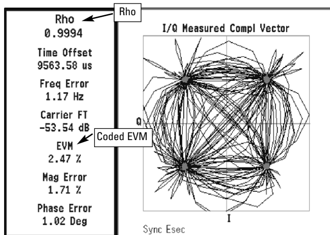
Figure 9. Rho and coded EVM measurement on a cdma2000 SR1 pilot signal
