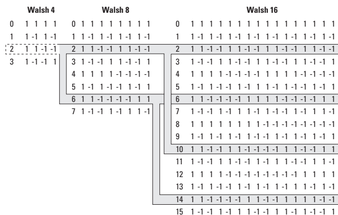
Figure 10. Hadamard generation of Walsh codes. Effects of using variable-length Walsh codes for spreading. Using a Walsh 4 code (in dashed box) precludes using codes in shaded area
