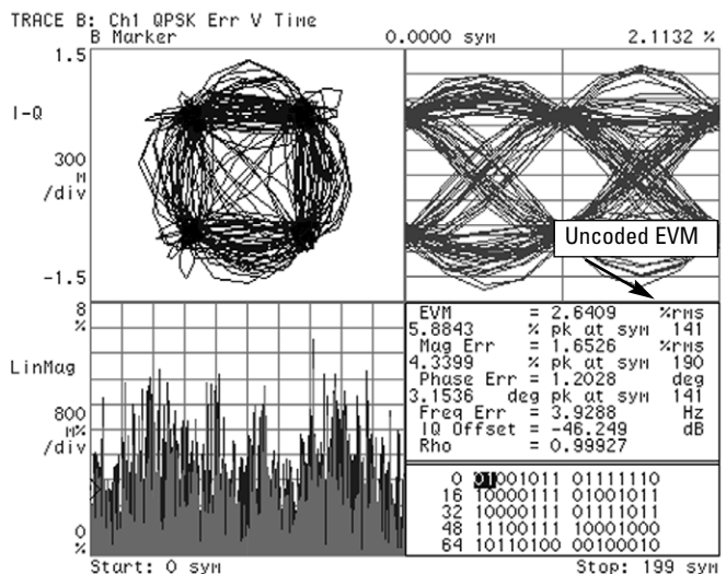
Figure 15. EVM (uncoded) on a cdma2000 SR1 reverse link signal with R-Pilot, R-FCH (RC3 at 9.6 kbps), and R-SCH 1 (RC3 at 307.2 kbps). All channels are at the same power level
